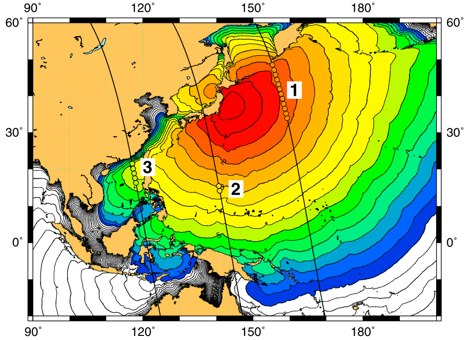
Figure 2. Expected crossing points (circles) between GOCE tracks and the gravity waves generated by the tsunami. Contour lines and color code represent the propagation time of the tsunami at the ocean surface computed by TTT (thick lines every hour). Circles filled with the tsunami propagation time color code are superimposed on the satellite tracks (black lines) in order to indicate the gravity wave crossing areas. The three crossing events are numbered in chronological order.
