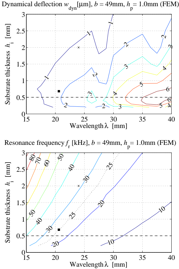
Figure 5: Contour lines of equal dynamical deflection in (a) and equal resonance frequency in (b) found by the numerical model for h_p = 1.0 \text{ mm} and Q = 54 . The square shows the optimum ( \lambda^* = 20.60 \text{ mm} , h_i^* = 0.683 \text{ mm} , w_{\text{dyn}} = 1.8417 \mu\text{m} , f_r = 25.04 \text{ kHz} ). The original plate indicated by the cross has \lambda = 24.00 \text{ mm} , h_i = 2.00 \text{ mm} , w_{\text{dyn}} = 1.151 \mu\text{m} , f_r = 31.17 \text{ kHz}
