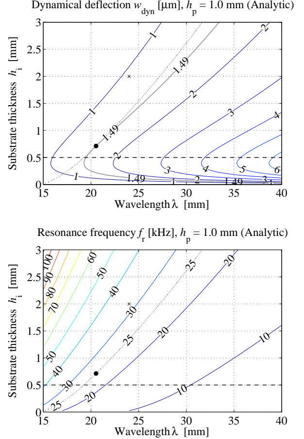
Figure 4: Contour lines of equal dynamical deflection in (a) and equal resonance frequency in (b) found by the analytical model for h_p = 1.0 mm and Q = 54 . The black circle shows the optimum ( \lambda^* = 20.54 mm, h_i^* = 0.712 mm, w_{\text{dyn}} = 1.4908 \mu\text{m} , f_r = 25.00 kHz), and the cross shows the original plate ( \lambda = 24.00 mm, h_i = 2.00 mm, w_{\text{dyn}} = 1.070 \mu\text{m} , f_r = 32.13 kHz). The dotted line indicates the minimal frequency of 25 kHz and the dashed line indicates the minimal resonator thickness of 0.5 mm. An additional contour line is added at w_{\text{dyn}} = 1.4908 \mu\text{m} to indicate the points with equal deflection as the optimum.
