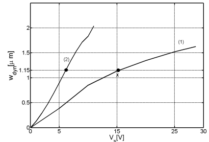
Figure 19: Measured dynamical deflection as a function of the supply voltage V_s (1) is for the plate P1 ( h_p = 1.0\text{mm} , h_i = 0.75\text{mm} , \lambda^* = 20.56\text{mm} ) and (2) is for P2 ( h_p = 0.5\text{mm} , h_i = 0.5\text{mm} , \lambda^* = 15.66\text{mm} ). The cross indicates the dynamical deflection of the original tactile plate
