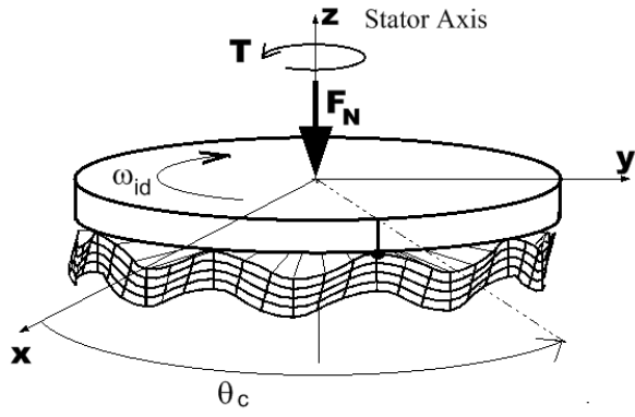
Fig. 1. Vibrating stator and the rotor pressed on it.
