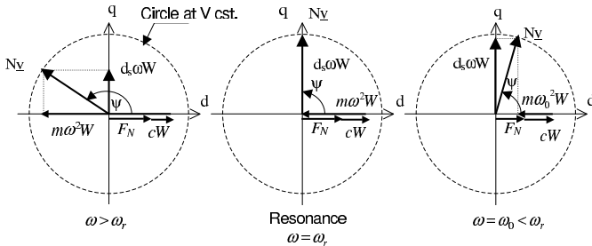
Fig. 3. Vector representation of steady-state operations in the rotating reference frame; T = 0 .
