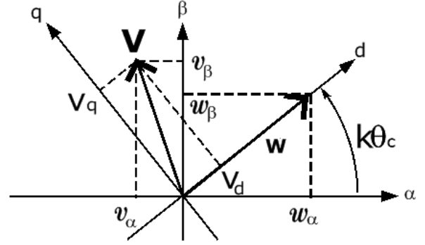
Fig. 2. Instant values of the stationary waves and voltages and the equivalent complex phasors \underline{w} and \underline{v} .
