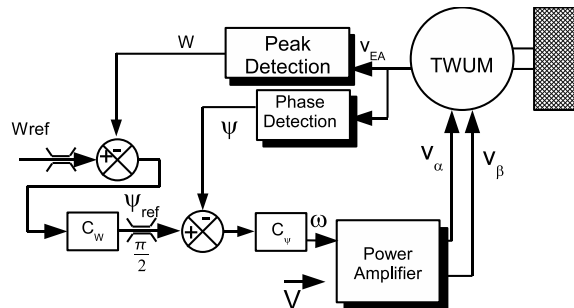
Fig. 15. Control in a rotating reference frame.
