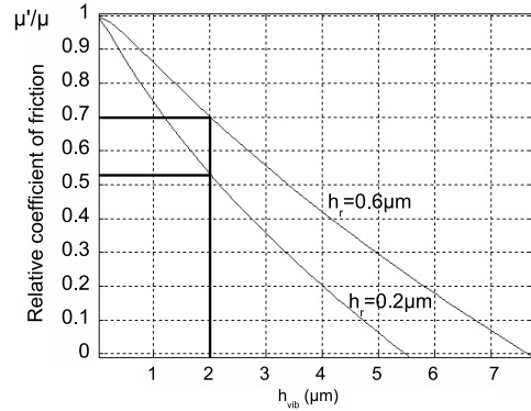
Fig. 5. The relative coefficient of friction as a function of the amplitude of vibration for F_f = 0.5\text{N} and for h_r = 0.2\mu\text{m} and h_r = 0.6\mu\text{m} .
