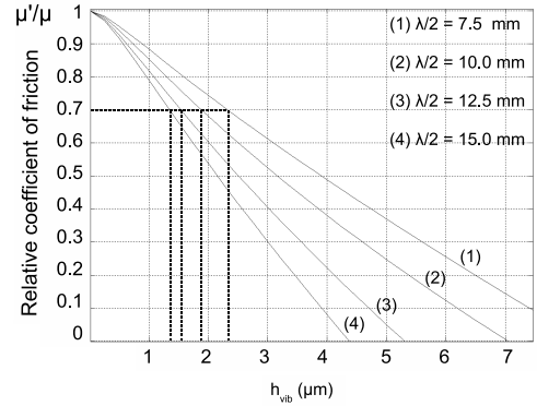
Fig. 11. The relative coefficient of friction as a function of the amplitude of vibration for F_f = 0.5\text{N} , h_r = 0.6\ \mu\text{m} and for 4 values of \lambda/2 .
