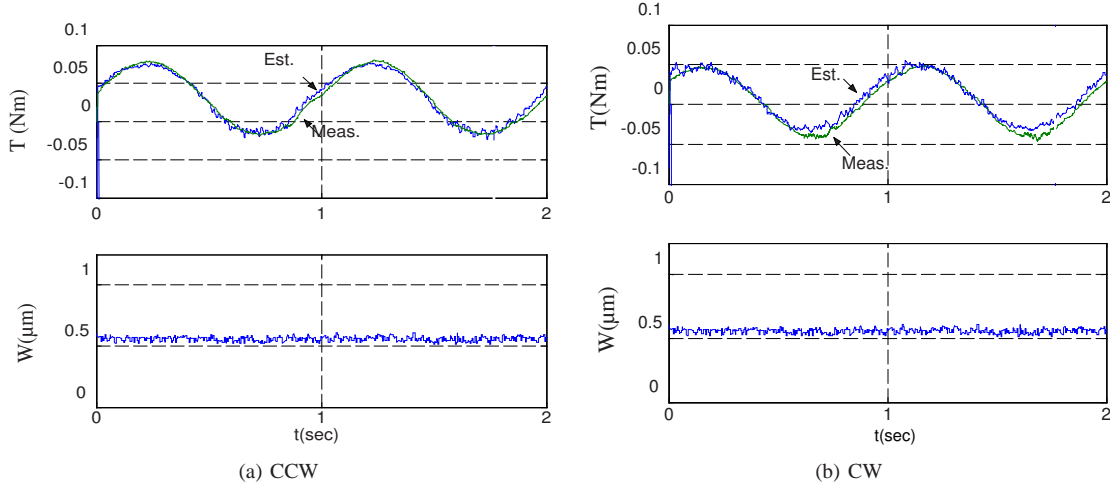
Fig. 10. Comparison between the actual load torque and the estimator's output for a constant travelling wave's amplitude.
