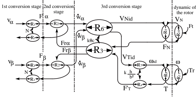
Fig. 3. Causal ordering graph of the TWUM.
