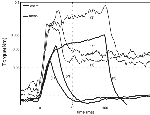
Fig. 15. Comparison of the output torque for several value of the limiting value of T: (1) T_{lim} = 0.03Nm , (2) T_{lim} = 0.05Nm , (3) T_{lim} = 0.065Nm .
