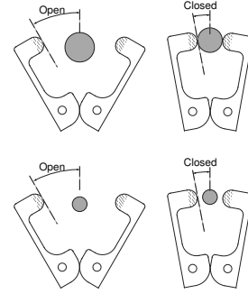
Fig. 12. Effect of a controlled position claw when the object is sufficiently big, and in the case where it is too small.
