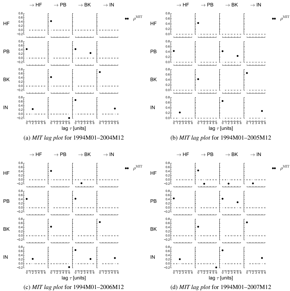
Figure 4: This is an alternative representation of the MIT Plots in Figure 3. A directed link “ \mathcal{A} \rightarrow^{\tau} \mathcal{B} ” means that \mathcal{B} is influenced by \mathcal{A} at lag(s) \tau . The existence of a dot at a particular lag \tau of sector \xi on the plots located on the diagonals indicates an autoregressive link of the form \xi_{t-\tau} \rightarrow \xi_t , which we denote as “ \xi_t \rightarrow^{\tau} \xi_t ”. Contemporaneous links can be read from the plots by observing dots at where \tau = 0 . The vertical axes represent the MIT coupling strength of the linkages.
