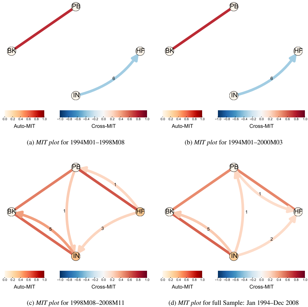
Figure 6: A directed link “ \mathcal{A} \rightarrow^\tau \mathcal{B} ” means that \mathcal{B} is influenced by \mathcal{A} at lag(s) \tau . The existence of a dot at a particular lag \tau of sector \xi on the plots located on the diagonals indicates an autoregressive link of the form \xi_{t-\tau} \rightarrow \xi_t , which we denote as “ \xi_t \rightarrow^\tau \xi_t ”. Contemporaneous links can be read from the plots by observing dots at where \tau = 0 . The vertical axes represent the MIT coupling strength of the linkages. We define time windows: 1994M01–1998M08, 1994M01–2000M03, 1998M08–2008M11, based on the distance matrix plot in Figure (5).
