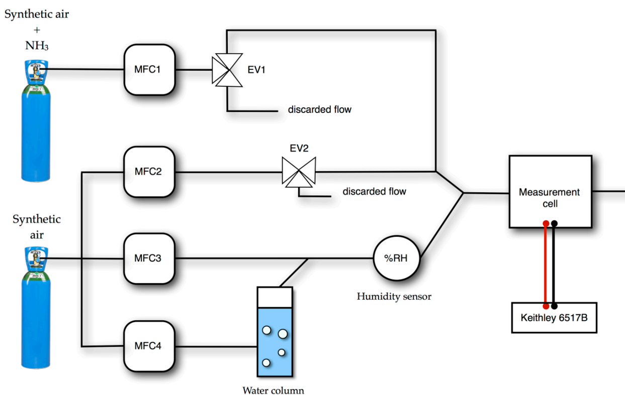
Figure 1. Scheme of the ammonia workbench.
