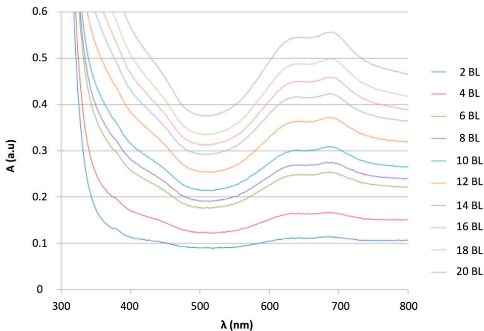
Figure 8. (PANI/CuTsPc) n (E5) absorption spectrum from 300 to 800 nm against the BL number.
