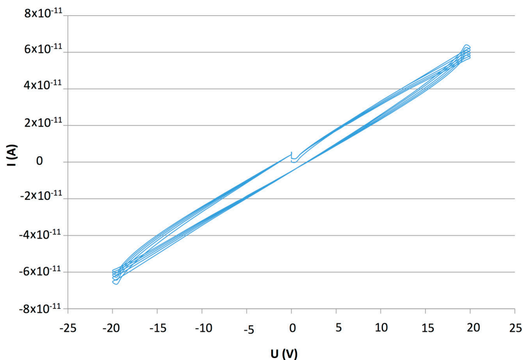
Figure 6. I-V characteristic of the (PDDA/s-CoPc) 15 device (E4), between −25 V to +25 V.
