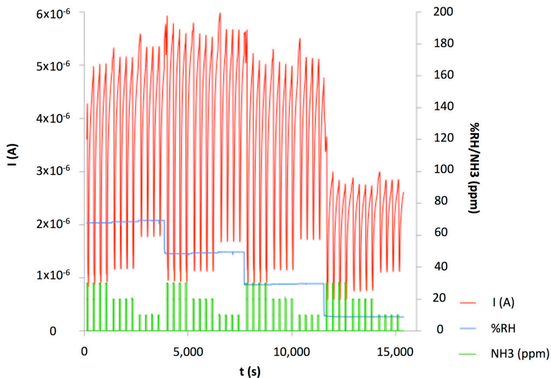
Figure 11. Ammonia/humidity exposure/recovery of a (\text{PANI}/\text{CuTsPc})_{20} device (E5) at 30, 20 and 10 ppm ammonia, with 70% to 10% RH, polarized at 1 V.
