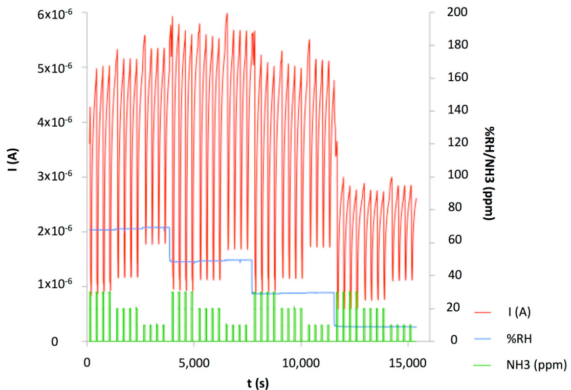
Figure 11. Ammonia/humidity exposure/recovery of a (PANI/CuTsPc) 20 device (E5) at 30, 20 and 10 ppm ammonia, with 70% to 10% RH, polarized at 1 V.
