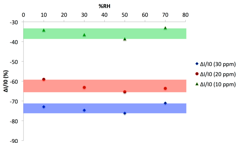
Figure 15. Relative response ( \Delta I/I_0 ) of a (\text{PANI}/\text{CuTsPc})_{20} device (E5) to \text{NH}_3 as a function of the Relative Humidity, as calculated from four 0.25/1 min exposure/recovery cycles. From bottom to top, the \text{NH}_3 concentration is 30, 20 and 10 ppm. The green, red and blue bands show the range of the relative response for respectively 10, 20 and 30 ppm \text{NH}_3 .
