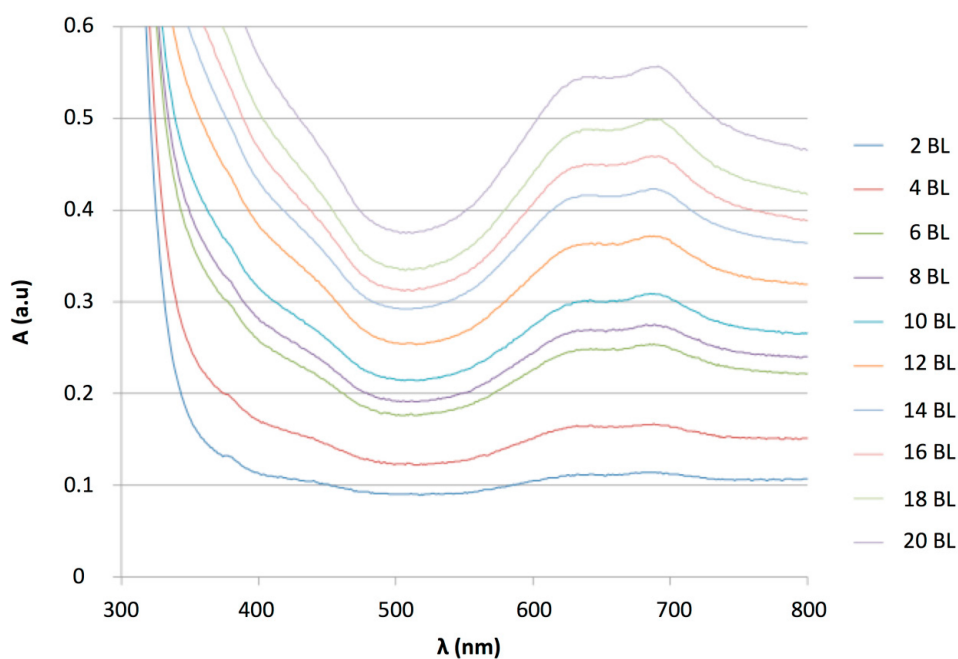
Figure 8. (PANI/CuTsPc) n (E5) absorption spectrum from 300 to 800 nm against the BL number.
