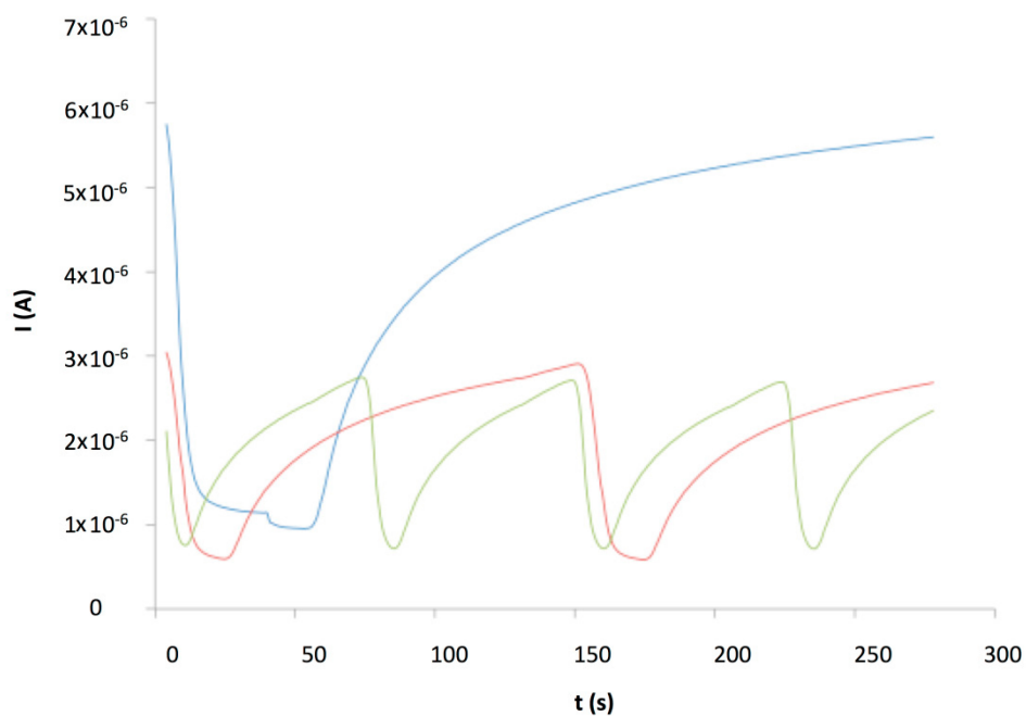
Figure 14. Current versus time of a (PANI/CuTsPc) 20 device (E5) exposed to 30 ppm NH 3 under 50% RH, with different exposure/recovery times, namely 1 min/4 min ( blue ), 0.5 min/2 min ( red ) and 0.25 min/1 min ( green ).
