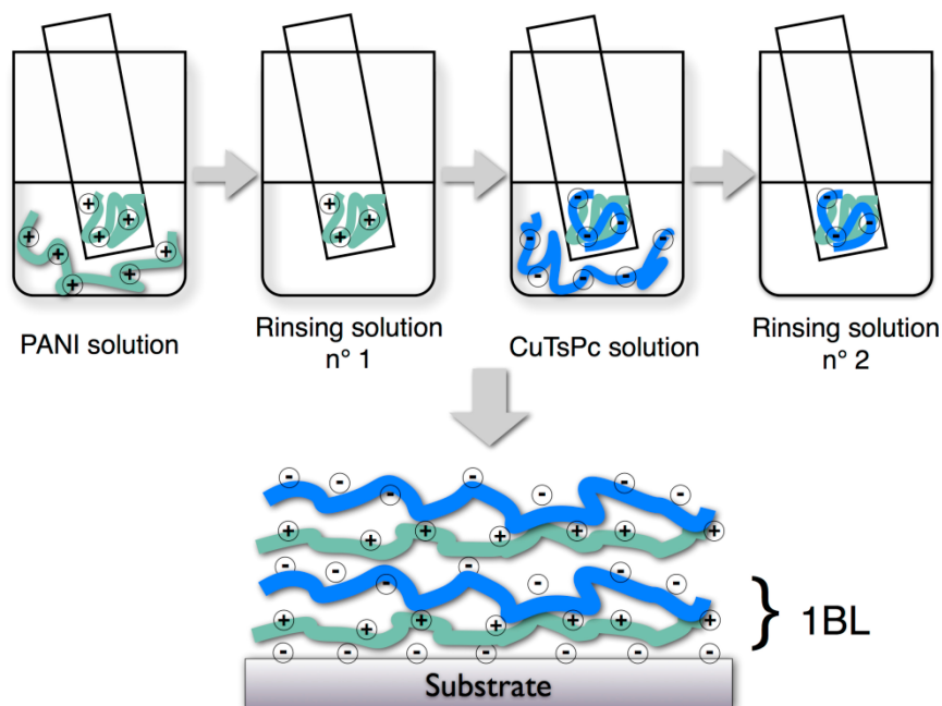
Figure 7. Scheme of the LBL process for PANI/CuTsPc films.
