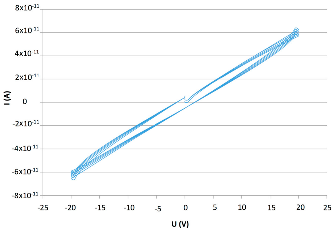
Figure 6. I-V characteristic of the (PDDA/s-CoPc) 15 device (E4), between −25 V to +25 V.
