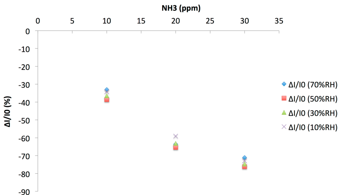
Figure 12. Relative response ( \Delta I/I_0 ) of a (\text{PANI}/\text{CuTsPc})_{20} device (E5) as a function of the \text{NH}_3 concentration at various RH values, as calculated from four 0.25 min/1 min exposure/recovery cycles.
