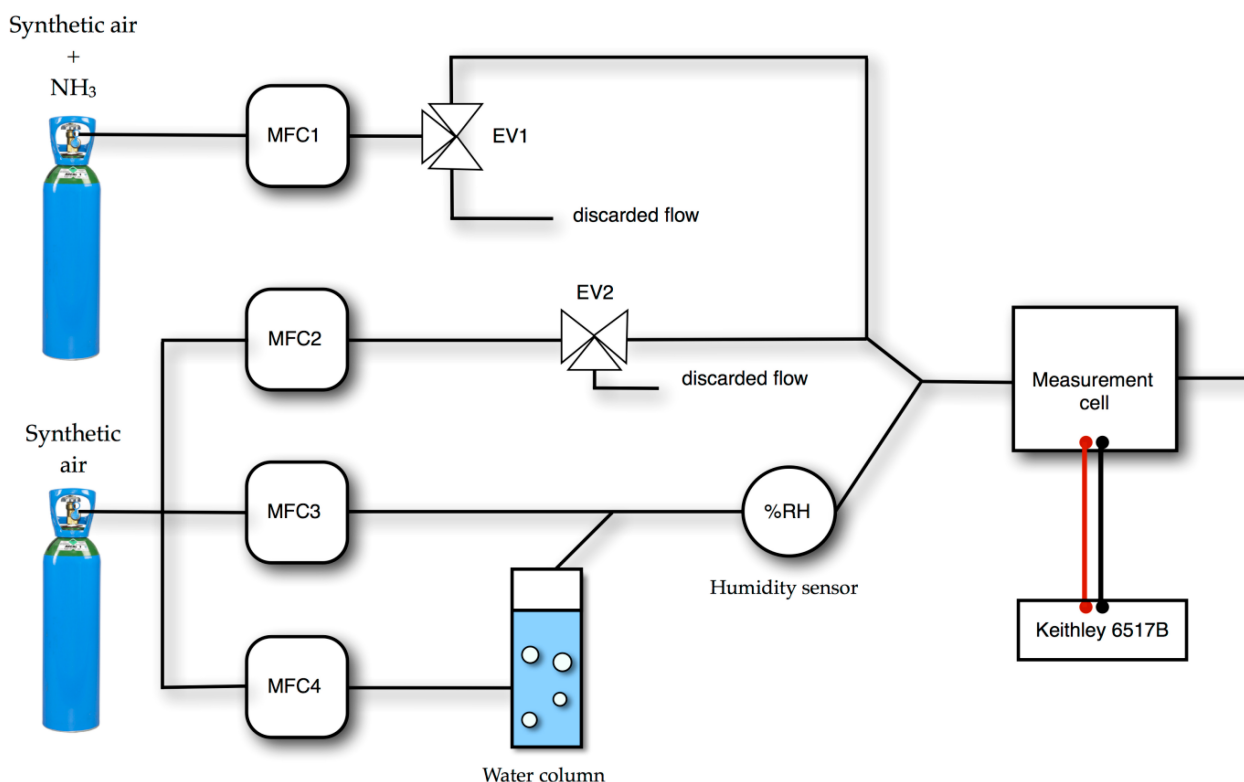
Figure 1. Scheme of the ammonia workbench.
