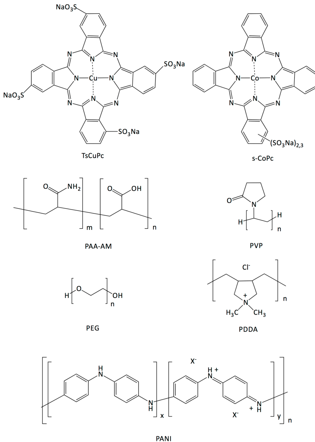
Figure 2. Structural formulas of compounds used in this study.
