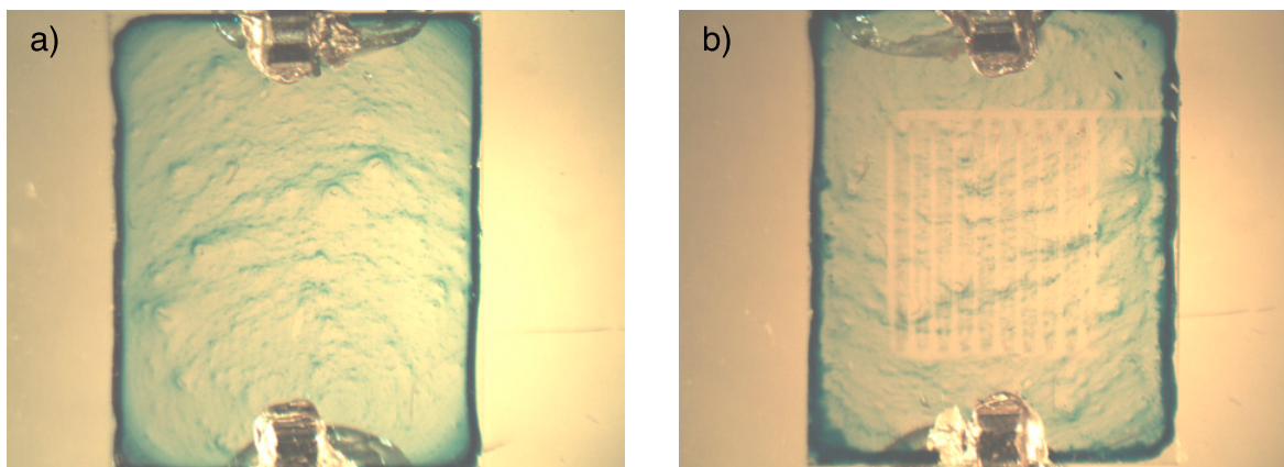
Figure 4. PVP resistor before humidity exposure (a); and after humidity exposure (b).
