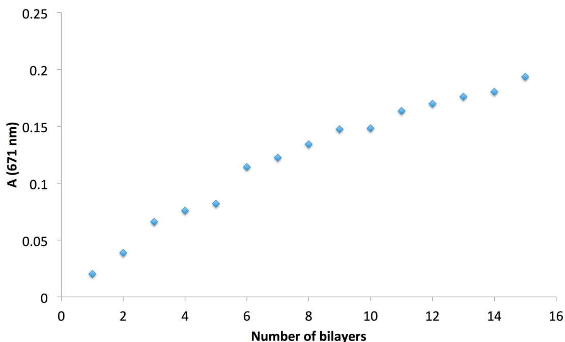
Figure 5. Absorbance measured at 671 nm against the number of PDDA/ s -CoPc bilayers.
