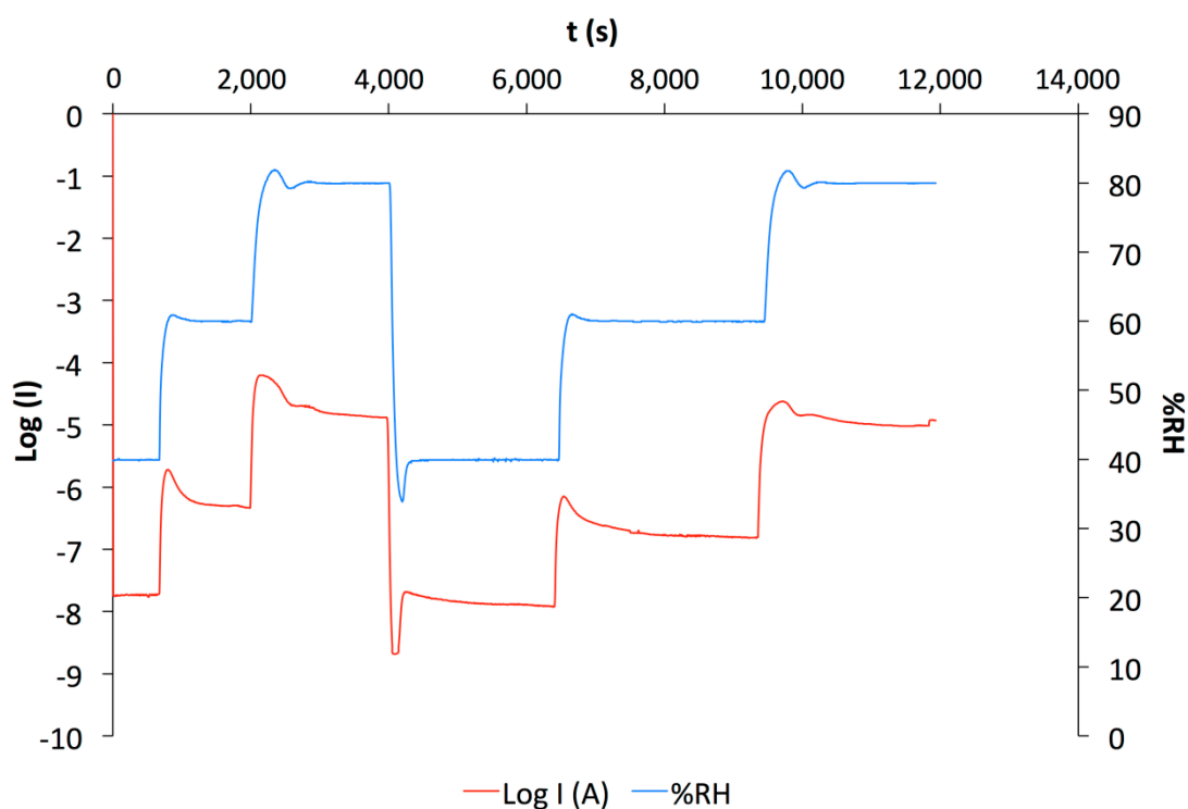
Figure 3. Humidity exposure experiment performed on s-CoPc/PEG sample (E2).
