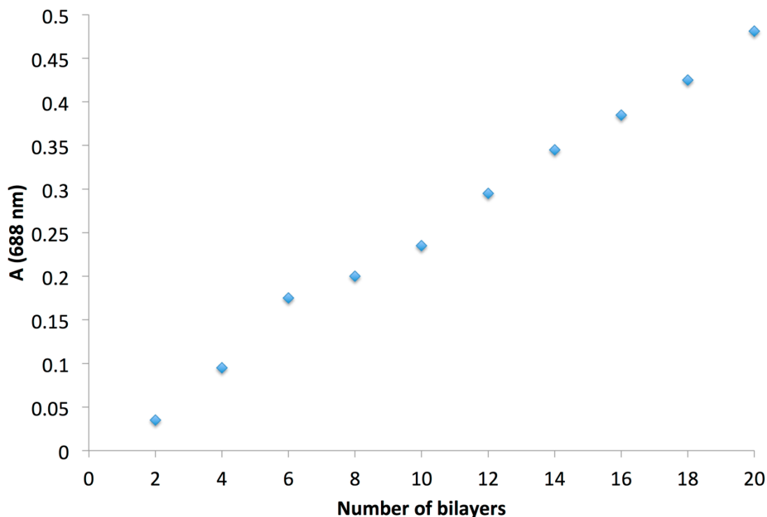
Figure 9. Absorbance measured at 688 nm, with the baseline correction, against the number of (PANI/CuTsPc) n bilayers (E5).
