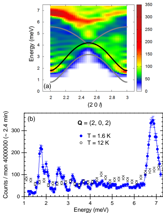
FIG. 7: (Color online) Inelastic scattering intensity map obtained from a series of \mathbf{Q} -constant energy scans measured at T = 1.6 K. The solid black line is the new fit to the lowest mode of the series, E_1^T , based on the assumption that its dispersion follows the lower boundary 2E_0^T of the two spinon continuum in the purely 1D case. The dashed black line comes from the folding of the previous dispersion due to the inter-chain couplings. Only the lower boundary of the continuum for the pure 1D model is plotted in this figure (grey solid line), the upper one being above the measured energy range. The white dash-dotted lines materialize the splitted anti-crossing branches (phenomenological fit).
