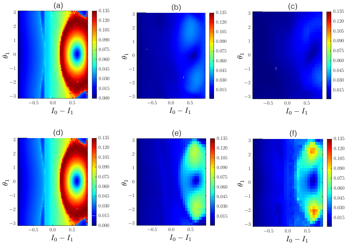
Figure 4: Variance of the wave packet position calculated between t = 0 and t = 800 from the GPE (left column), LD (center column), and THM (right column) with N = 30 (top row) and N = 400 (bottom row) and the same parameters as Fig. 1.
