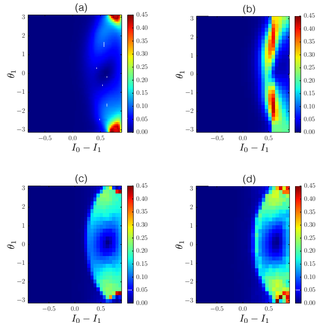
FIGURE 3: Spectral entropy distribution in phase space obtained by LD (left column) and by THM (right column) with N = 30 (top row) N = 400 (bottom row) and same parameters as Fig. 1. When N increases, the THM provides a quite good representation of the mean-field behavior for large N , and the phase-space structure of the many-body problem becomes similar to the Poincaré section obtained from the GPE, plot (a) of Fig. 1.
