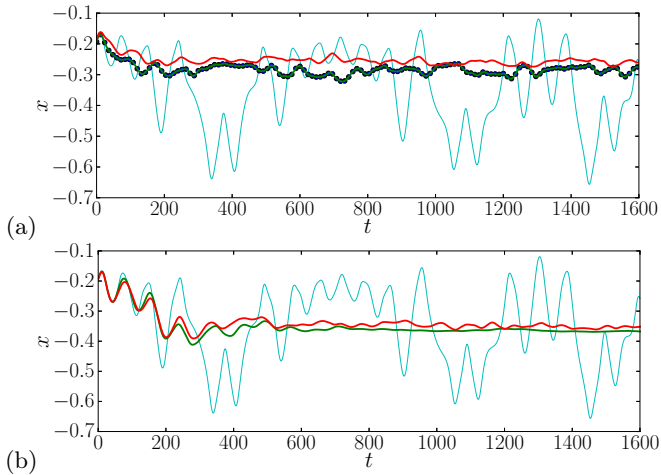
FIGURE 2: Evolution of the average position of a wave packet calculated with different methods : Gross-Pitaevskii equation (cyan), Lanczos diagonalization (green), and the truncated Husimi method (red), for (a) N = 30 and (b) N = 500 . In panel (a), we also represented by blue circles the result obtained by direct diagonalization of the full many-body problem, which is in perfect agreement with the result of the Lanczos method, illustrating the accuracy of the later. The initial state is a SU(3) coherent state with c_{-1} = \sqrt{0.5} , c_0 = \sqrt{0.25} and c_1 = i\sqrt{0.25} . Other parameters are gN = 0.2 , V_0 = 7 , F = 0.1 .
