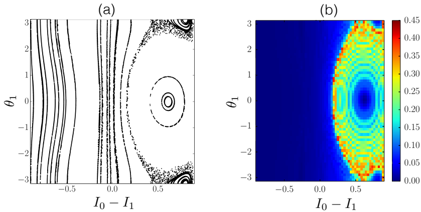
FIGURE 1: Quasiclassical chaos in a tilted lattice, obtained by integrating the Gross-Pitaevskii equation (4). (a) Poincaré section corresponding to I_{-1} = 0.1 , \theta_0 - \theta_{-1} = 0 . (b) Spectral entropy calculated between t = 0 and t = 800 . Parameters are V_0 = 5 , F = 0.25 , gN = 0.2 .
