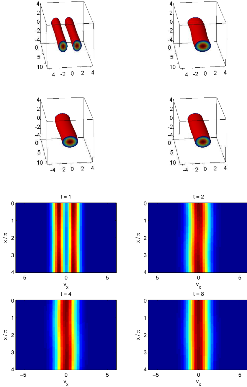
FIGURE 7. Two stream instability associated with Knudsen number \varepsilon = 10^{-4} at time t = 1, 2, 4, 8 . Top: 3D illustration; Bottom: projection in the x - v_x plane.
