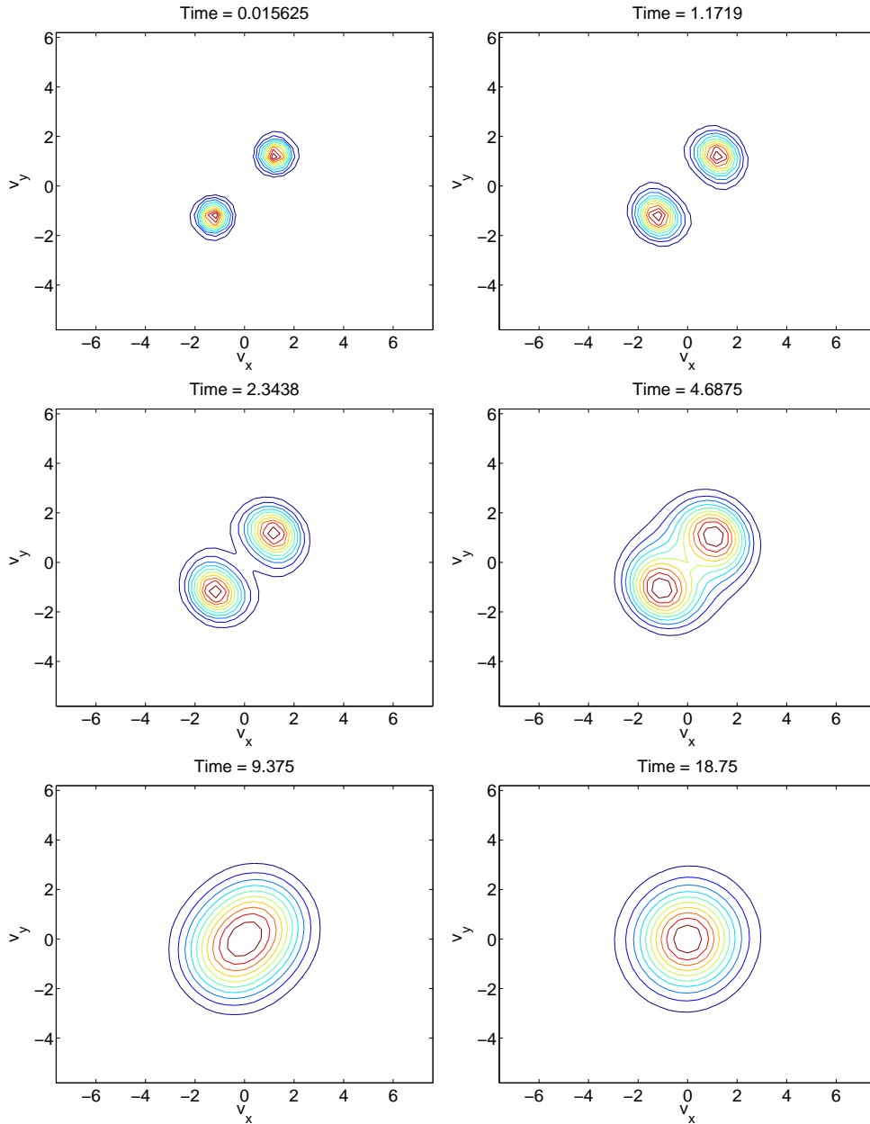
FIGURE 1. Time evolution of the level set of distribution function f , starting from the double peak distribution (4.2). A first order exponential Runge-Kutta method is used for the time integration.
