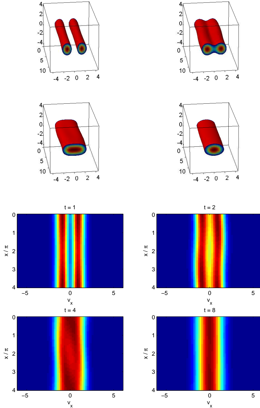
FIGURE 6. Two stream instability associated with Knudsen number \varepsilon = 1 at time t = 1, 2, 4, 8 . Top: 3D illustration; Bottom: projection in the x - v_x plane.
