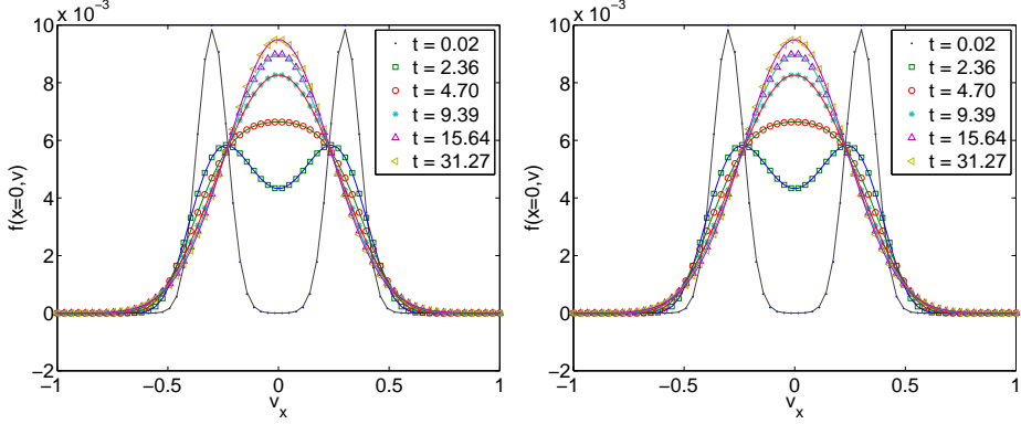
FIGURE 2. Time evolution of distribution function f(v_x, v_y = 0) at various time slot for Rosenbluth's test problem. Solid lines: reference solution computed by an explicit RK3 method with \Delta t = 1.0078 \times 10^{-4} . Markers: solution computed by exponential RK3 method (left) and third order IMEX-RK method (right) with \Delta t = 0.0156 .
