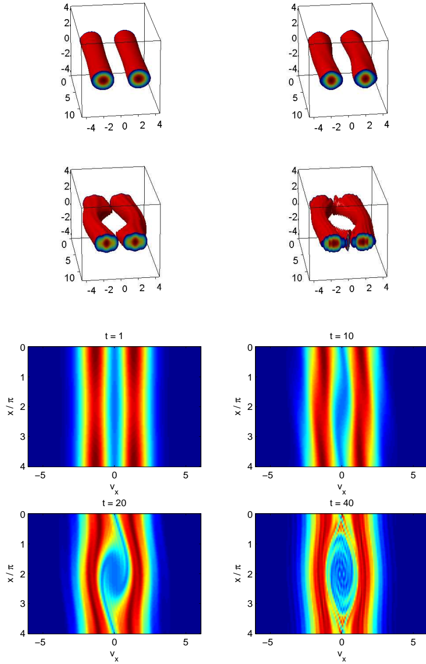
FIGURE 5. Two stream instability without collision at time t = 1, 10, 20, 40 . Top: 3D illustration; Bottom: projection in the x - v_x plane.
