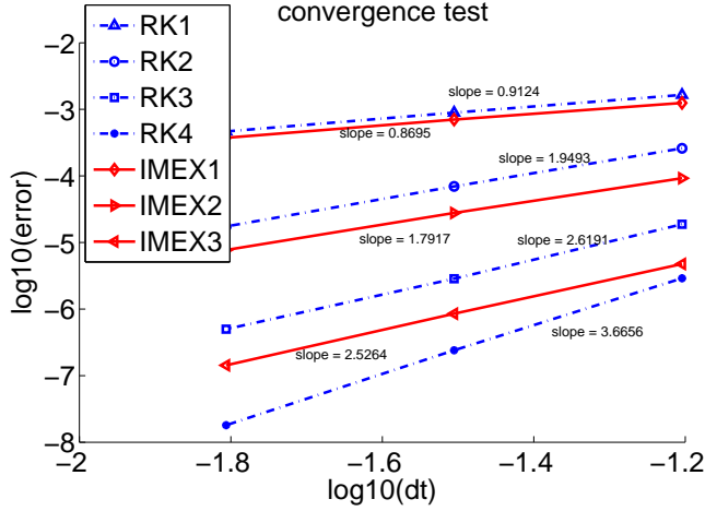
FIGURE 3. The convergence rates of the exponential Runge-Kutta methods (dotted line with markers) and of the IMEX-RK method (solid line with markers) for the homogeneous LFP equation with initial data (4.2) and (4.4).
