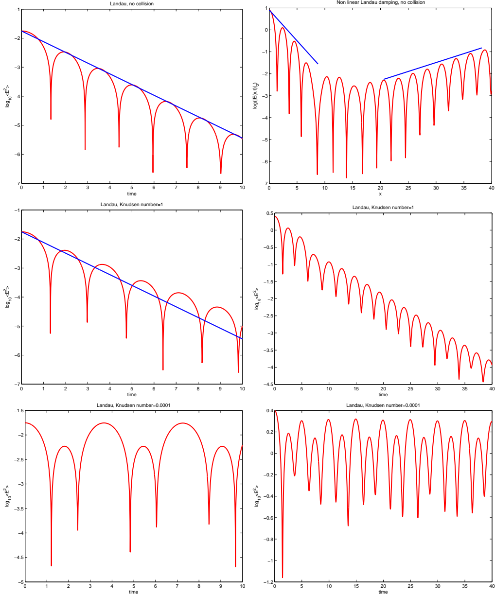
FIGURE 4. The linear Landau damping on the left and the non linear Landau damping on the right associated to different Knudsen numbers. The three figures, from top to bottom are for \varepsilon = \infty, 1 and 10^{-4} respectively.
