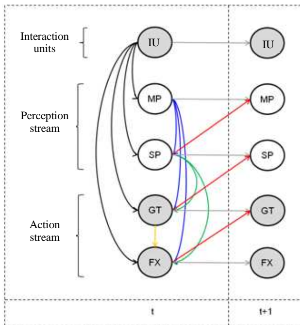
Figure 3: Dependency graph between interaction units, perception and action streams automatically inferred from “put-that-there” data for the DBN. Arrows of different colors (distinguishing intra- vs. inter-modality, intra- vs. inter-frame dependencies) cue significant dependencies between units and observations. Contrary to HMM, no latent states have been added here.
