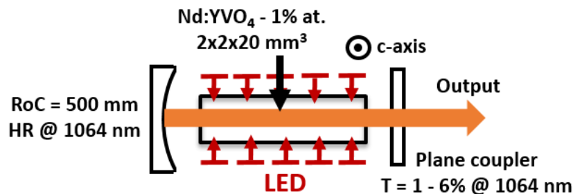
Figure 3. Experimental setup.
