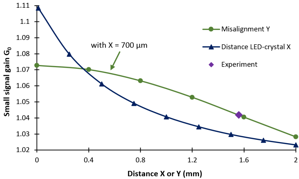
Figure 7. Evolution of the theoretical small signal gain G_0 as a function of the misalignment between the two LEDs (Y) and the distance between LEDs and the crystal (X). This calculations are used to estimate the misalignment Y in our experiment.
