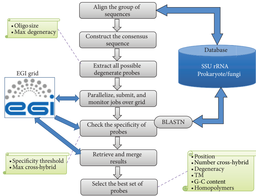
FIGURE 1: Summary of algorithm steps.
