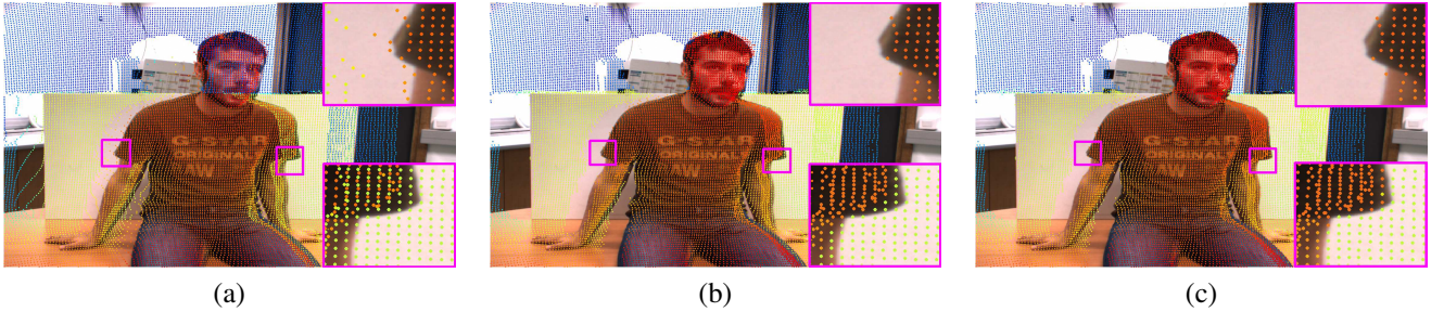
Fig. 2: (Best viewed on screen) (a) The mapping of depth data onto the left image causes artifacts in the presence of depth discontinuities. A cascade of (b) geometry-consistency and (c) color-consistency filters refines the sparse disparity map. Depth values are color-coded from red (close) to blue (far).
