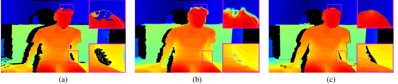
Fig. 3: (Best viewed on screen) Depth upsampling results using (a) triangulation-based interpolation [15] after cutting big triangles, (b) joint bilateral filter [34] and (c) our method. The depth values are color-coded from red (close) to blue (far), while black areas correspond to non-available values. The white edges in close-ups show the color edges of the image.
