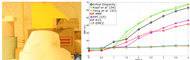
Fig. 9: Left image with superimposed depth map (left) and BMP curves (right) for the HR stereo pair Lampshade1 . The lower curves show the robustness of the proposed schemes to the noise of the initial depth map.
