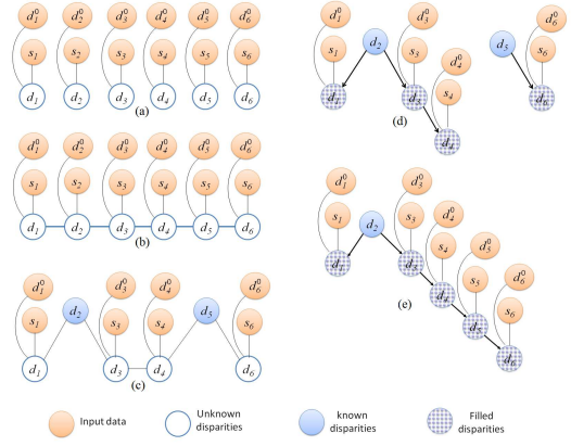
Fig. 8: Dependency network for (a) WTA and (b) MRF models in an 1D example. Initial and two final candidate graphs for the proposed scheme are shown in (c), (d) and (e) respectively.
