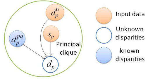
Fig. 5: The principal graph that is iteratively considered in our region-growing fusion method.
