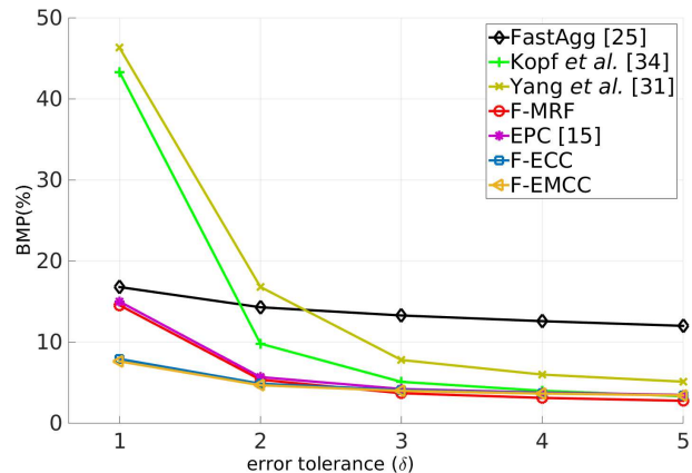
Fig. 10: The BMP error of fusion algorithms averaged over the eight test images as a function of the error tolerance \delta .
