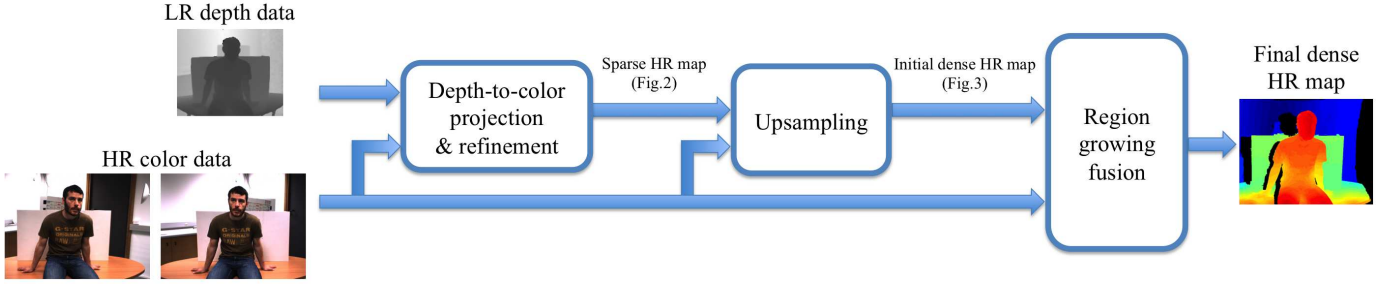
Fig. 1: The pipeline of the proposed depth-stereo fusion method. The low-resolution (LR) depth data are projected onto the color data and refined to yield a high-resolution (HR) sparse disparity map. Starting from these disparity seeds, an upsampling process provides an initial HR dense disparity map. Both the HR seeds and the initial dense disparity map are then used by the region-growing depth-stereo fusion to produce the final HR depth map. A prominent feature of our method is that fusion takes place at several data processing stages.
