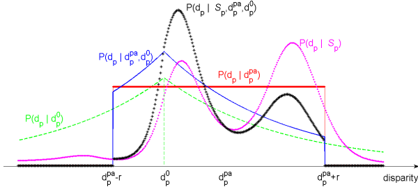
Fig. 6: An example of the probability distribution of d_p constrained by different observations.
