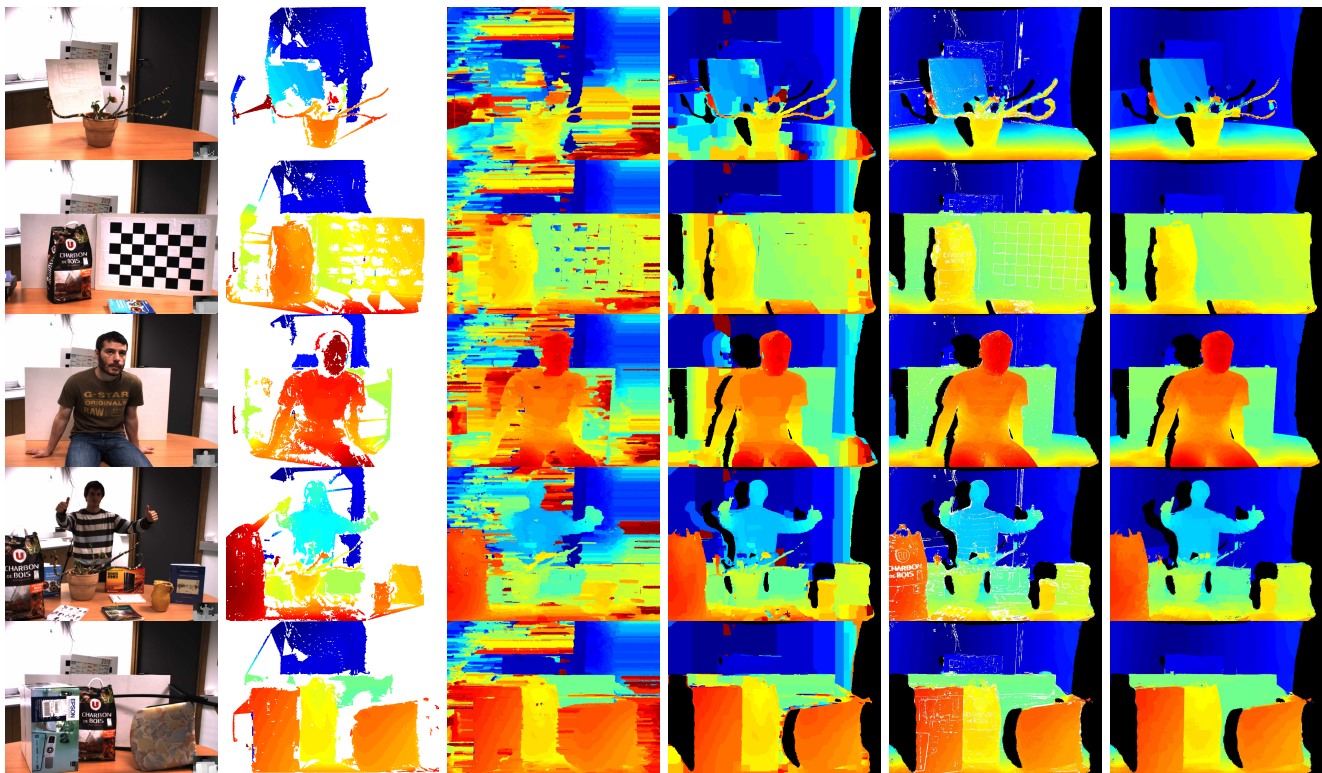
Fig. 13: HR images and disparity maps for MIXCAM dataset obtained by (from left to right) ELAS, FastAgg, F-MRF (GC), F-ECC, and F-ECC after post-processing.
