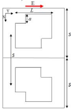
Fig. 4. Schematic for 2\times 1 unit-cell with opposite-notched DRA
