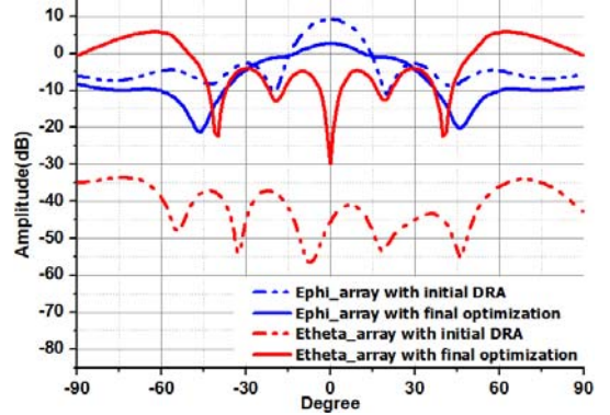
Fig. 11. Comparison of array with notched DRAs after final optimization and array with non-notch DRAs
