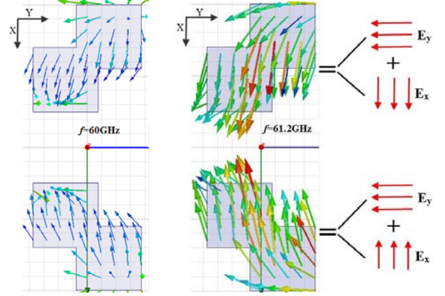
Fig. 5. E-field distribution for 2\times 1 unit-cell around 60\text{GHz}
