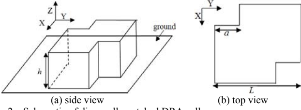
Fig. 2. Schematic of diagonally notched DRA cell
