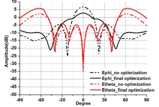
Fig. 10. E pattern comparison of initial dimension and final optimization( \phi=0 plane)
