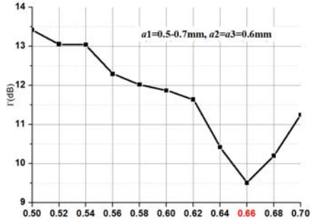
Fig. 9. \Gamma optimization of a_1
