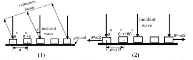
Fig. 1. (1) General working principle for passive repeater array based on DRA, (2) Proposed implementation for combined endfire/backfire radiation
