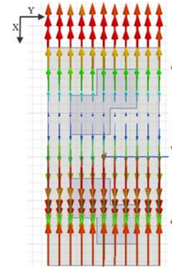
Fig. 6. E-field distribution of \text{TM}_{10} mode for incident wave
