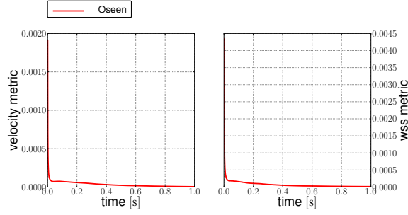
Figure 5: Fully implicit vs. Semi-implicit, \Delta t = 10^{-3} , inlet velocity v_{\text{in}} = 30 \times 10^{-3} \text{ m} \cdot \text{s}^{-1} .
