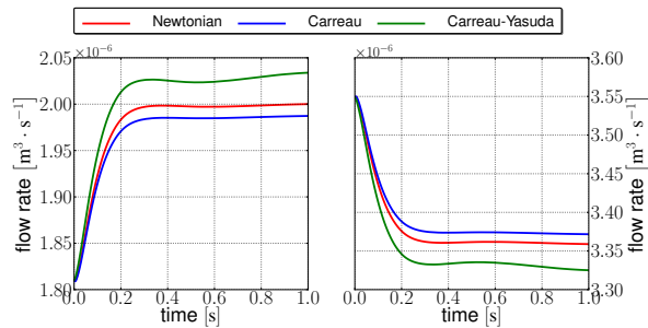
Figure 11: Flow rate measured at RIJV outlet (left) and LIJV outlet (right). Each result has been obtained with v_{\text{in}} = 30 \times 10^{-3} \text{ m} \cdot \text{s}^{-1} and free-traction outflow condition.
