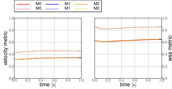
Figure 16: Effects of inlet velocity magnitude v_{\text{in}} . The reference solution for each level mesh is computed using v_{\text{in}} = 10 \times 10^{-3} \text{ m} \cdot \text{s}^{-1} . Continuous lines correspond to v_{\text{in}} = 20 \times 10^{-3} \text{ m} \cdot \text{s}^{-1} and dashed lines to v_{\text{in}} = 30 \times 10^{-3} \text{ m} \cdot \text{s}^{-1} .
