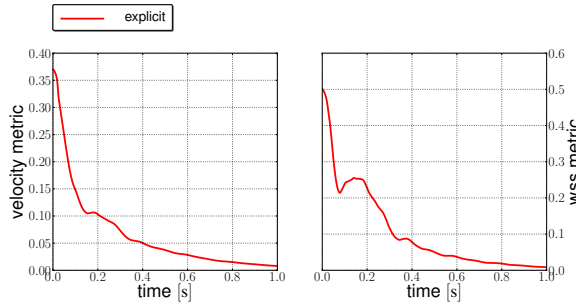
Figure 6: 3D-0D implicit vs. explicit, inlet velocity v_{\text{in}} = 30 \times 10^{-3} \text{ m} \cdot \text{s}^{-1} .
