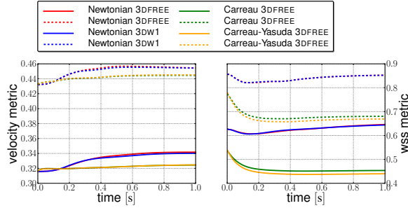
Figure 17: Effects of inlet velocity magnitude v_{\text{in}} . The reference solution for each model is computed by using v_{\text{in}} = 10 \times 10^{-3} \text{ m} \cdot \text{s}^{-1} . Continuous lines correspond to v_{\text{in}} = 20 \times 10^{-3} \text{ m} \cdot \text{s}^{-1} and dashed lines to v_{\text{in}} = 30 \times 10^{-3} \text{ m} \cdot \text{s}^{-1} .
