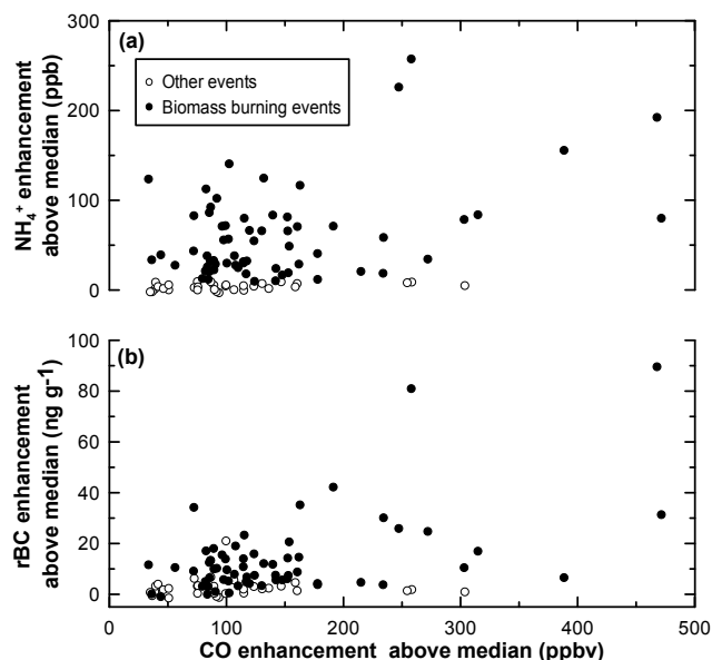
Figure 6. CO concentration enhancements above median values for the 96 spikes selected along the NEEM-2011-S1 record, as a function of \text{NH}_4^+ (a) and rBC (b) concentrations. Both \text{NH}_4^+ and rBC are shown as enhancement levels above their corresponding median. Ice layers enriched with pyrogenic aerosols (closed circles) are identified when [\text{NH}_4^+] > 18 ppb (Savarino and Legrand, 1998).
