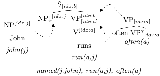
Fig. 1. Derivation and Semantics for “John often runs”
