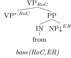
Fig. 6. Deriving Smaller from Larger Trees
