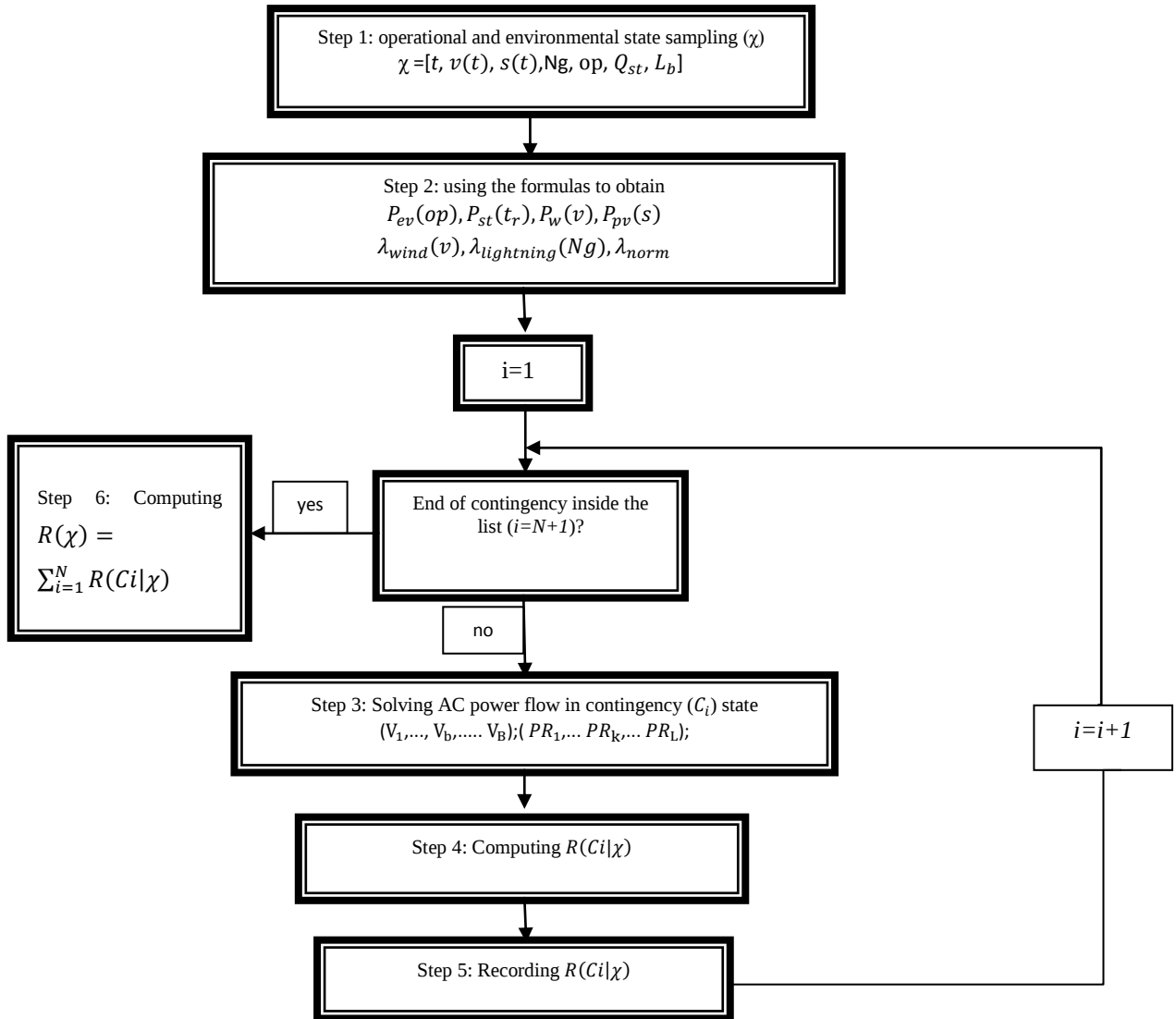
Fig.3 Flow chart of a single MC run
