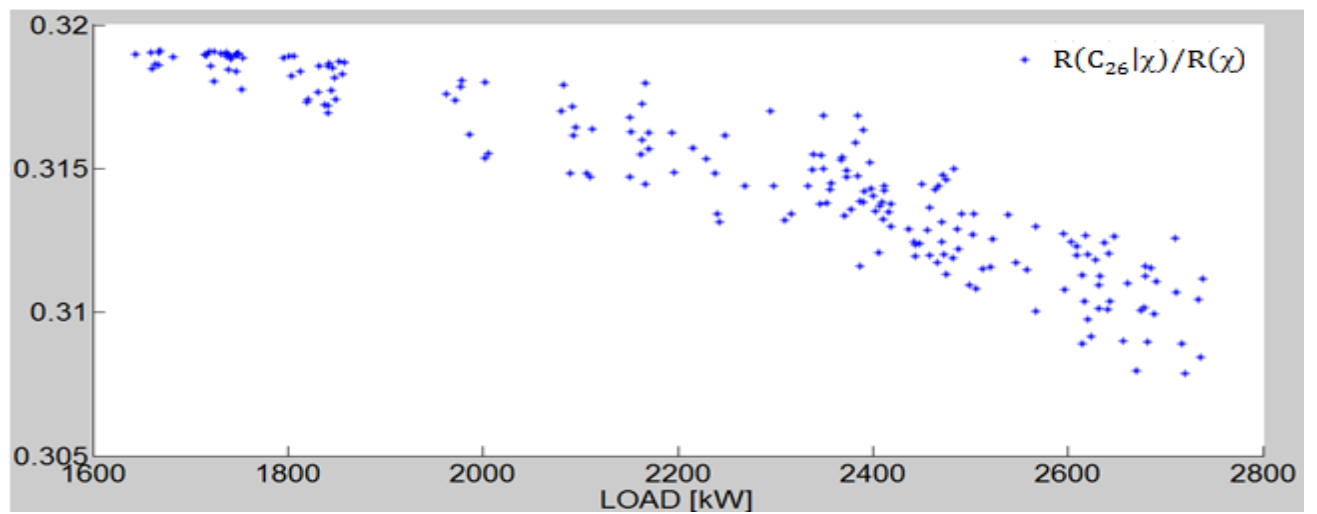
Fig.12(b) R(C_{26}|\chi)/R(\chi) for various load levels
