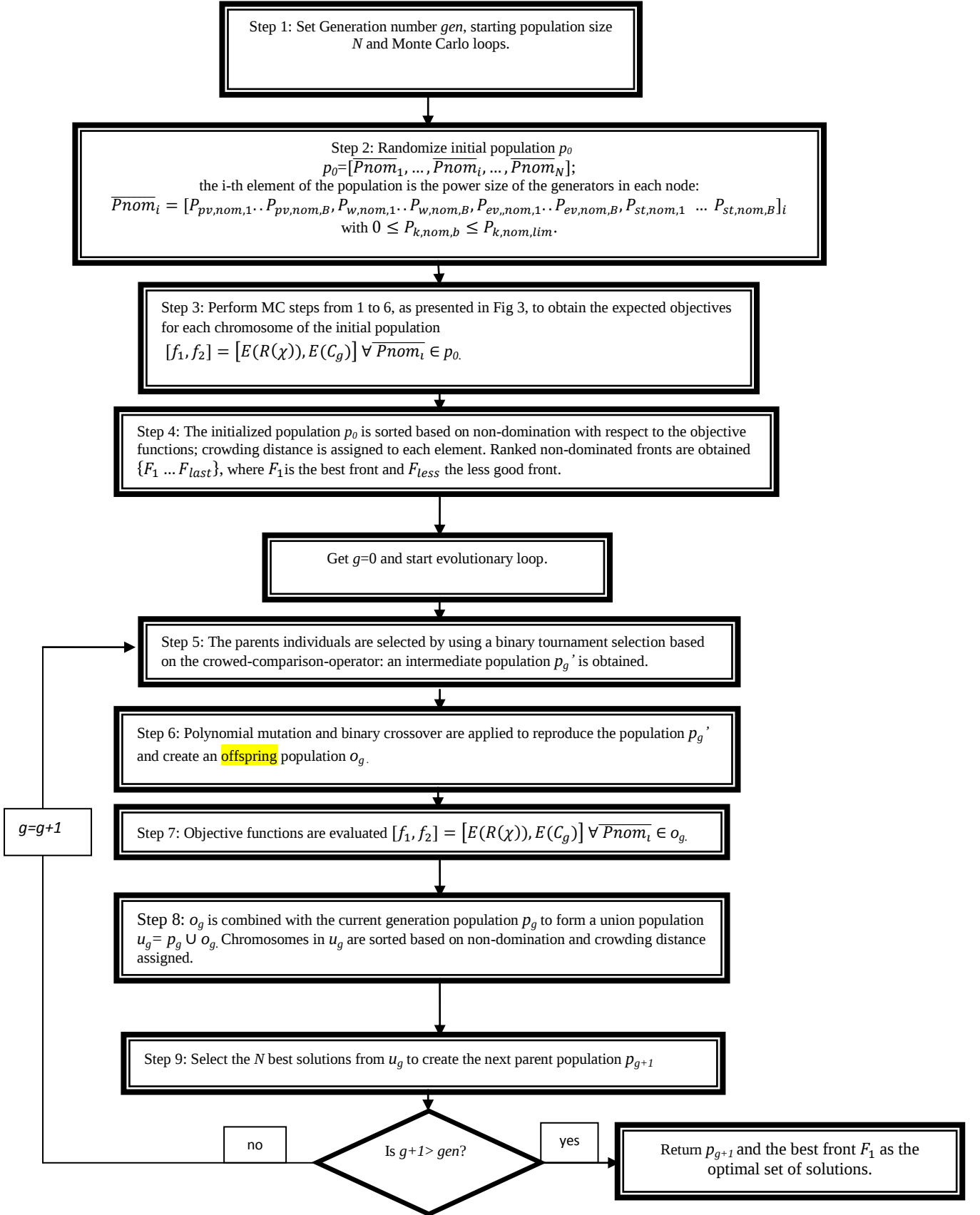
Fig.4 Flow chart of RBMOO-NSGA-II
