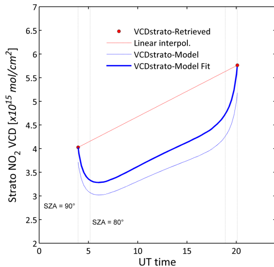
Figure 4. Representation of the retrieved stratospheric NO 2 VCDs at 90° SZA sunrise and sunset for reference day 174 (Sect. 3.4.1) and fit of the NO 2 diurnal cycle modelled with the photochemical model PSCBOX.
