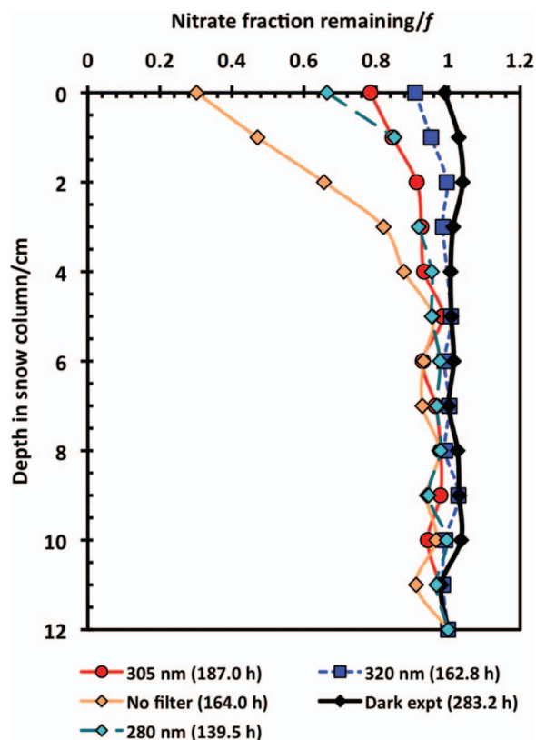
FIG. 3. Nitrate concentration profile (fraction of nitrate remaining, f ) versus depth in the snow column plotted for the experiments conducted using different filters. “0” represents the side of the snow column closest to the lamp.
