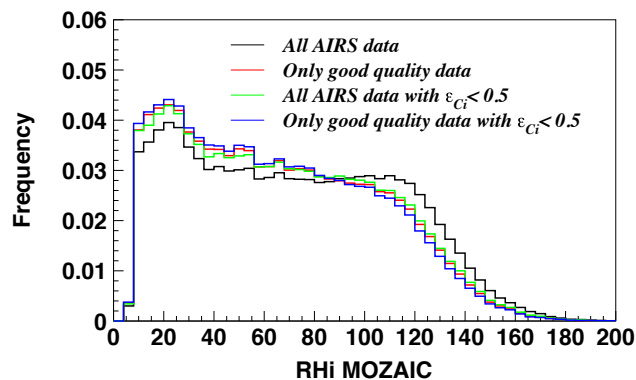
Fig. 1. Distributions of relative humidity seen from MOZAIC \text{RH}_{\text{M}} in collocation with AIRS data (all qualities combined) or only with good quality AIRS data for all cloud types and when removing the thickest cirrus clouds with \epsilon_{\text{clid}} > 0.5 .
