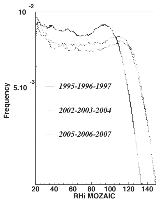
Fig. 5. Distributions of relative humidity seen by MOZAIC \text{RH}_{\text{M}} for the years 1995-1996-1997 compared to distributions for 2002-2003-2004 and 2005-2006-2007.
