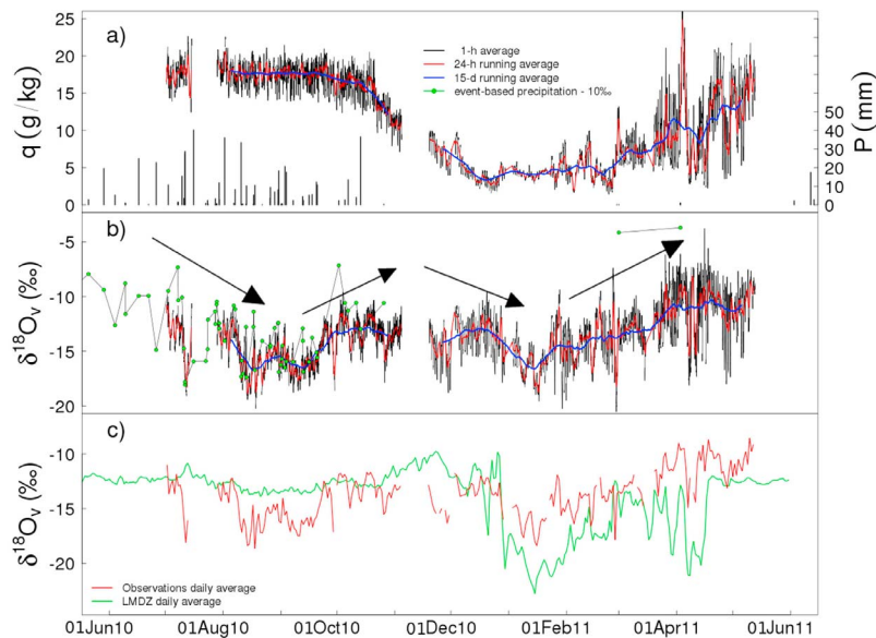
Figure 1. Temporal evolution from June 2010 to May 2011 of (a) Specific humidity q (g/kg) along with event-based rain-fall amount P (mm). From 23 April to 26 October 2010, 66 rain events were collected (total amount of 523.8 mm, precipitation varied from 0.1 mm to 40.3 mm); (b) \delta^{18}\text{O}_v (‰): black, red and blue lines are hourly averages, 24-h and 15-days running averages respectively. Intense power cuts (from 15 to 28 July 2010) and maintenance period (from 5 to 18 Nov 2010), where a new automated calibration system was set up, are responsible for the 2 major gaps. Event-based ( \delta^{18}\text{O}_p - 10 ) (‰) are in green dots; and (c) \delta^{18}\text{O}_v (‰) in our observations (red line) and in LMDZ-iso (green dotted line).
