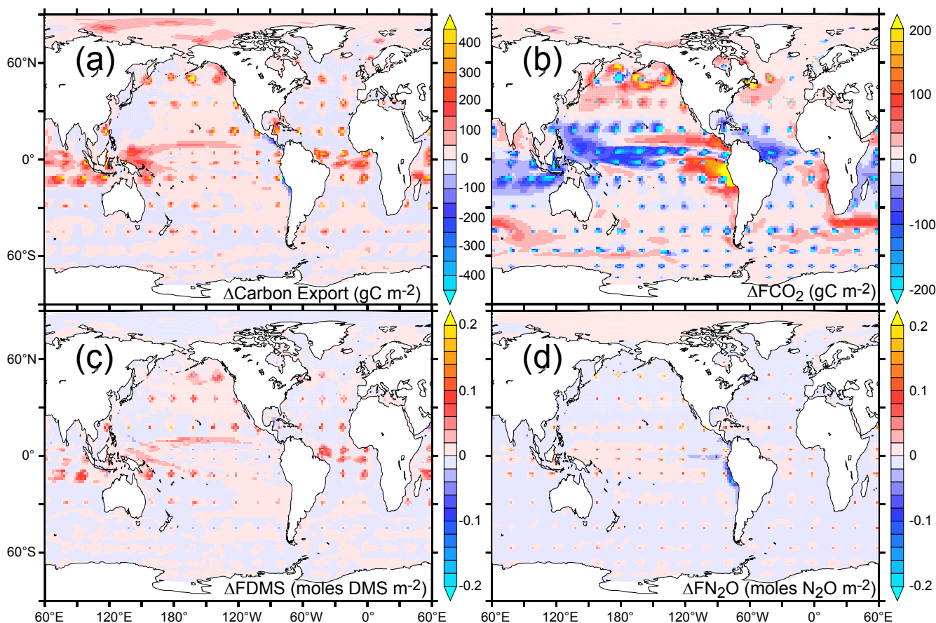
Fig. 2. Spatial maps of the cumulative anomaly (over 20 years) in (a) carbon export ( \text{gC m}^{-2} ), (b) ocean CO 2 uptake (FCO 2 , \text{gC m}^{-2} ), (c) ocean to atmosphere DMS flux (FDMS, moles DMS \text{m}^{-2} ), and (d) ocean to atmosphere N 2 O flux (FN 2 O, moles N 2 O \text{m}^{-2} ).
