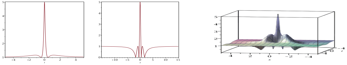
Figure 2. Solution to NLS, N=2 , to the left v(x, 0) ; in the center v(0, t) ; to the right v(x, t) .
