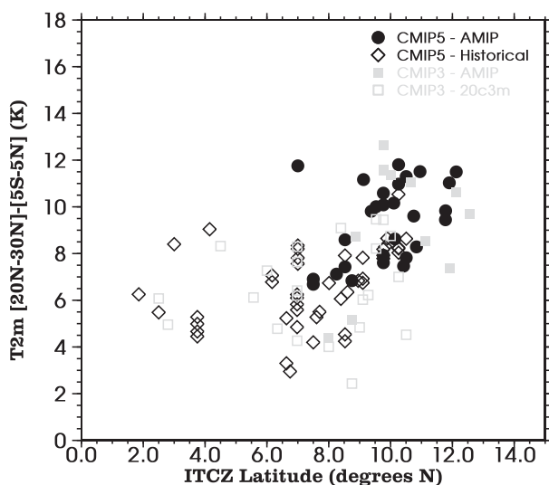
FIG. 5. Scatterplot of the ITCZ position versus the meridional temperature gradient between the Gulf of Guinea and the Sahara desert. The ITCZ latitude corresponds to the position during JAS of maximum precipitation averaged over 10°W–10°E. The JAS temperature gradient is computed as the difference between (20°–30°N, 10°W–10°E) and (5°S–5°N, 10°W–10°E): CMIP5 AMIP (black circles), CMIP5 Historical (open diamonds), CMIP3 AMIP (gray squares), and CMIP3 20C3M (open squares).
