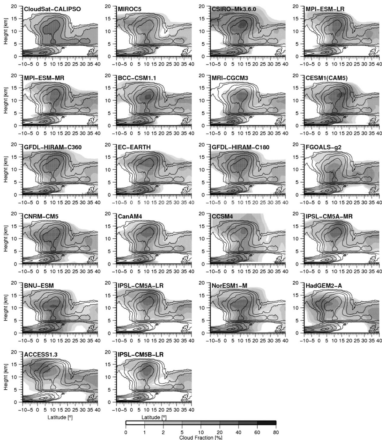
FIG. 8. Latitude–height plots of cloud fraction averaged between 10^{\circ}\text{W} and 10^{\circ}\text{E} for the JAS season for the years 2006–10 for the CloudSat – CALIPSO dataset and 1979–2008 for the models. Models are organized (top left)–(bottom right) from the warmest over the Sahara ( 20^{\circ} – 30^{\circ}\text{N} , 10^{\circ}\text{W} – 10^{\circ}\text{E} ) to the coldest.
