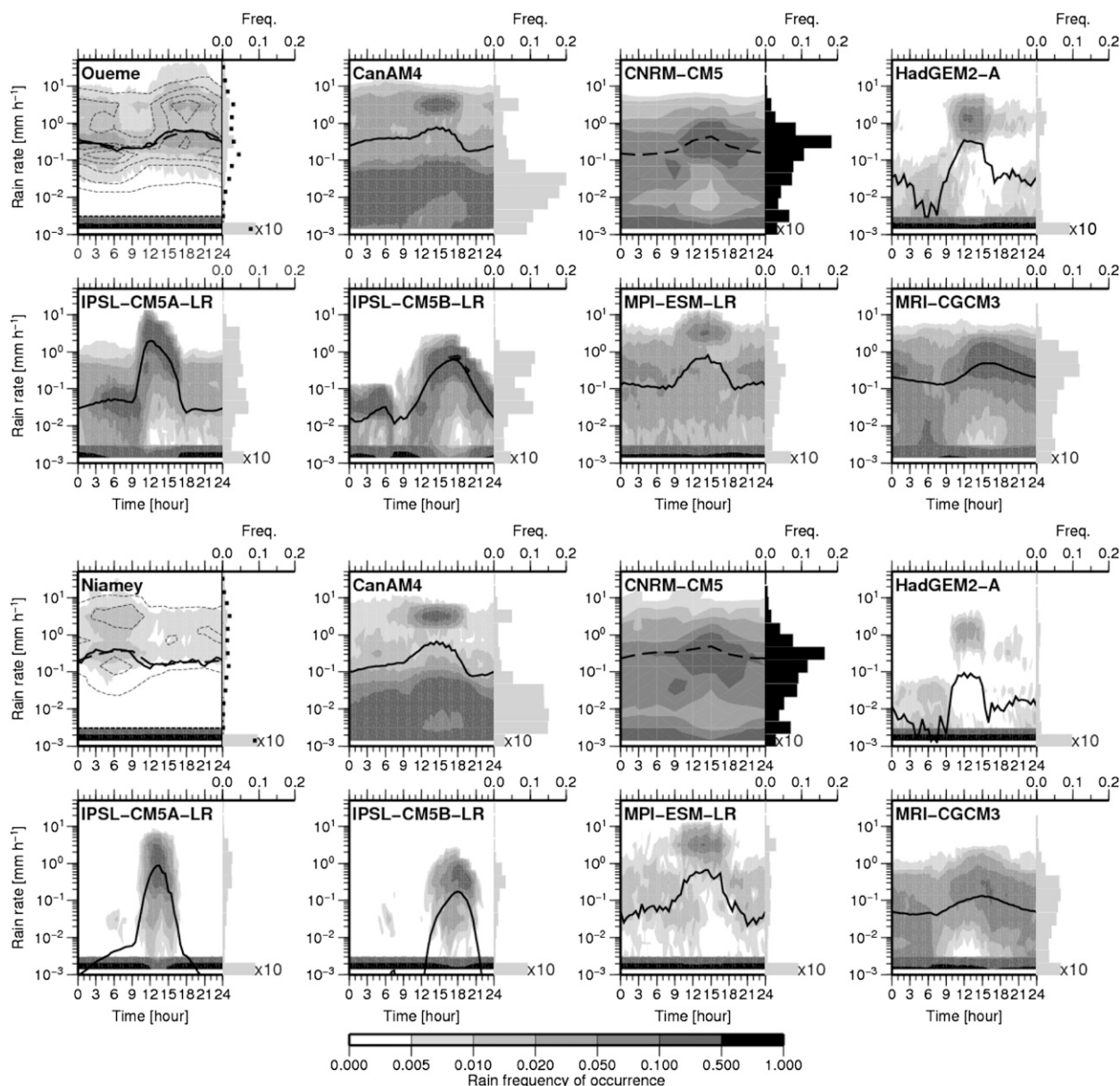
FIG. 17. Mean August diurnal cycle of precipitation intensity distribution (including null values). Periods used are 1979–2008 for the models, 1999–2011 for the Ouémé site ( 9.5^{\circ}\text{N} , 2^{\circ}\text{E} ), and 1989–2011 for the Niamey site ( 13.5^{\circ}\text{N} , 2.2^{\circ}\text{E} ). The distribution is based on 30-min samples. The mean diurnal cycle of rainfall intensity is superimposed (black line). The diurnal cycle of precipitation intensity distribution is also shown (dashed lines) but using 3-hourly samples for comparison with the CNRM-CM5 model.
