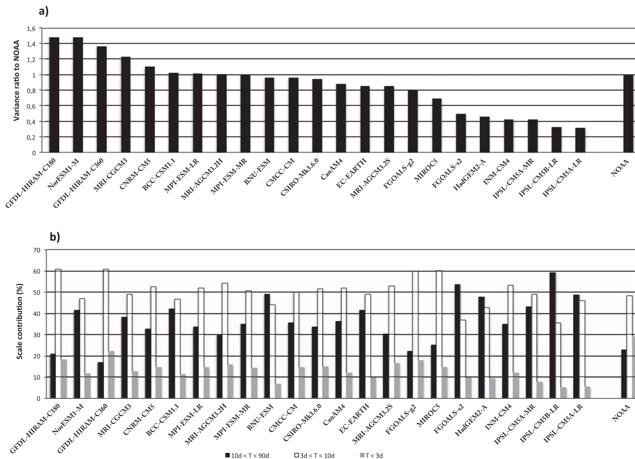
FIG. 15. (a) Variance of OLR in the 1–90-day band averaged over the domain ( 5^{\circ} – 20^{\circ} N, 10^{\circ} W– 10^{\circ} E) for the JAS season from 1979 to 2008. Values are normalized by the NOAA OLR variance. (b) Distribution of the OLR intraseasonal variance (%) across the 1–3-day (gray bars), 3–10-day (white bars), and 10–90-day (black bars) time scales.
