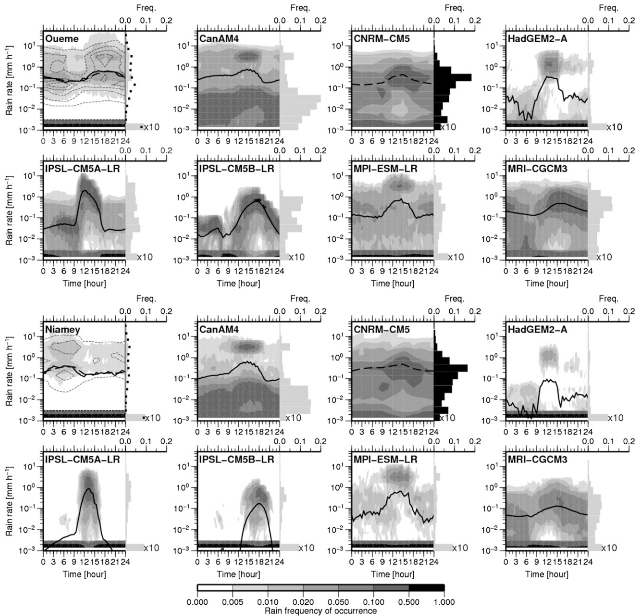
FIG. 17. Mean August diurnal cycle of precipitation intensity distribution (including null values). Periods used are 1979–2008 for the models, 1999–2011 for the Ouémé site (9.5°N, 2°E), and 1989–2011 for the Niamey site (13.5°N, 2.2°E). The distribution is based on 30-min samples. The mean diurnal cycle of rainfall intensity is superimposed (black line). The diurnal cycle of precipitation intensity distribution is also shown (dashed lines) but using 3-hourly samples for comparison with the CNRM-CM5 model.
