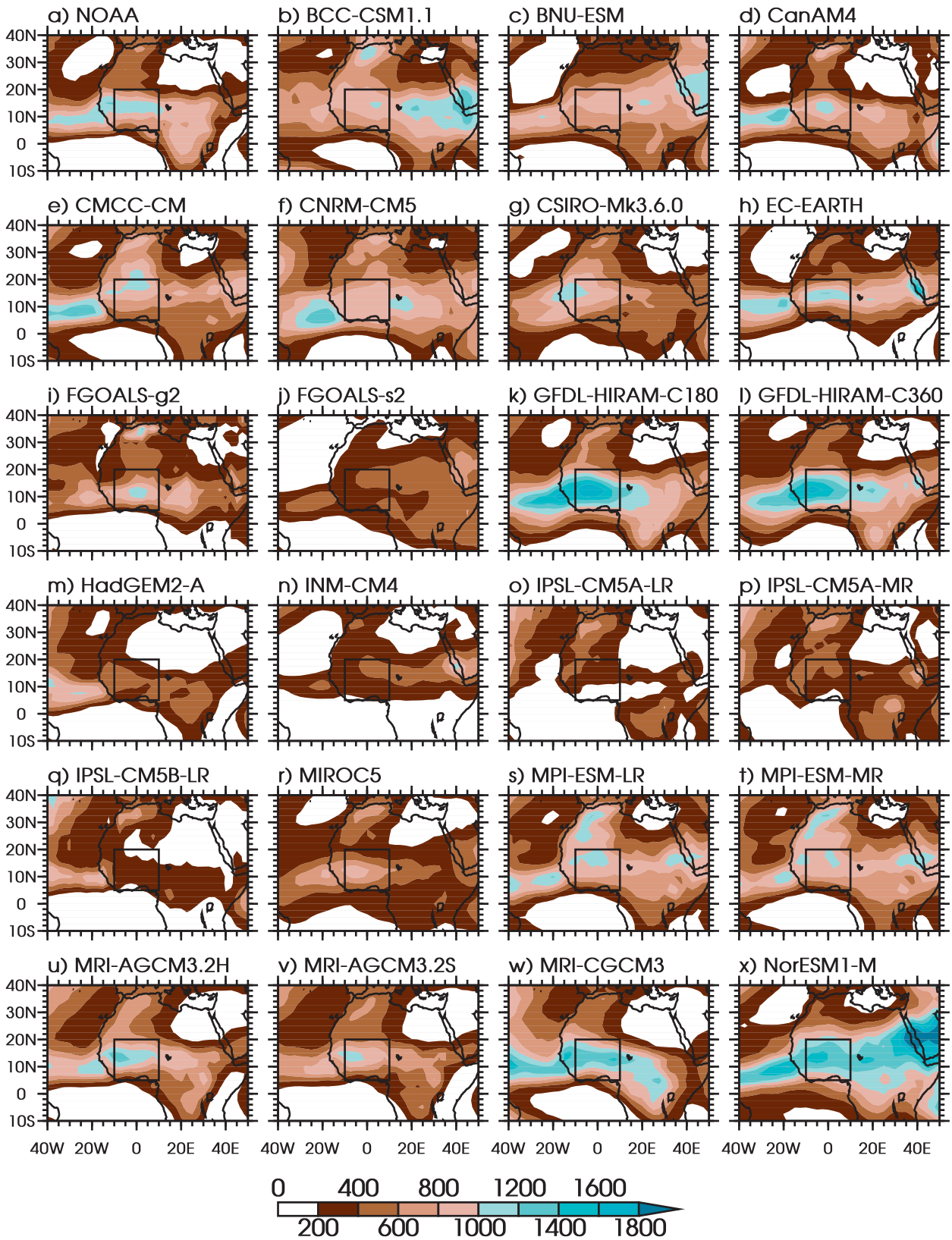
FIG. 14. Variance of OLR in the 1–90-day band ( W^2 m^{-4} ) for the JAS season from 1979 to 2008. The daily OLR of the CMIP5 models was regridded onto the National Oceanic and Atmospheric Administration (NOAA) OLR grid ( 2.5^\circ \times 2.5^\circ ), before computing filtered anomalies and their variance.
