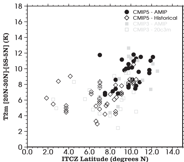
FIG. 5. Scatterplot of the ITCZ position versus the meridional temperature gradient between the Gulf of Guinea and the Sahara desert. The ITCZ latitude corresponds to the position during JAS of maximum precipitation averaged over 10^{\circ}\text{W} – 10^{\circ}\text{E} . The JAS temperature gradient is computed as the difference between ( 20^{\circ} – 30^{\circ}\text{N} , 10^{\circ}\text{W} – 10^{\circ}\text{E} ) and ( 5^{\circ}\text{S} – 5^{\circ}\text{N} , 10^{\circ}\text{W} – 10^{\circ}\text{E} ): CMIP5 AMIP (black circles), CMIP5 Historical (open diamonds), CMIP3 AMIP (gray squares), and CMIP3 20C3M (open squares).
