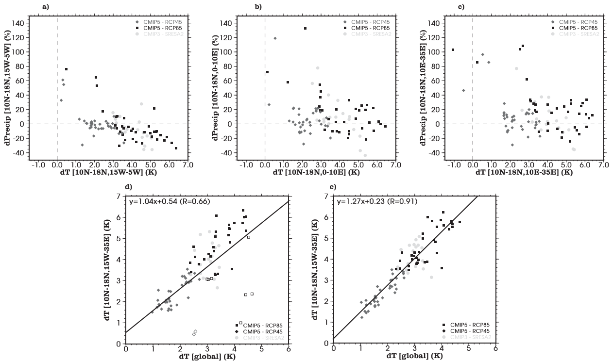
FIG. 2. (a) Climate precipitation projections (%) plotted against those of 2-m temperature (K) averaged over the westernmost Sahel grid box ( 10^{\circ} – 18^{\circ} N, 15^{\circ} – 5^{\circ} W) shown in Fig. 1a. The differences are computed between the periods 2071–2100 and 1971–2000 for the JAS season for the CMIP3 SRES A2 scenario, and the CMIP5 RCP4.5 and RCP8.5 scenarios. (b) As in (a), but for the central West Sahel grid box ( 10^{\circ} – 18^{\circ} N, 0^{\circ} – 10^{\circ} E). (c) As in (a), but for the central–eastern Sahel grid box ( 10^{\circ} – 18^{\circ} N, 10^{\circ} – 35^{\circ} E). (d) Climate projections of global 2-m temperature plotted against 2-m temperature averaged over the Sahel domain ( 10^{\circ} – 18^{\circ} N, 15^{\circ} W– 35^{\circ} E); white squares are projections of precipitation change >25\% . (e) As in (d), but for the MAM season.
