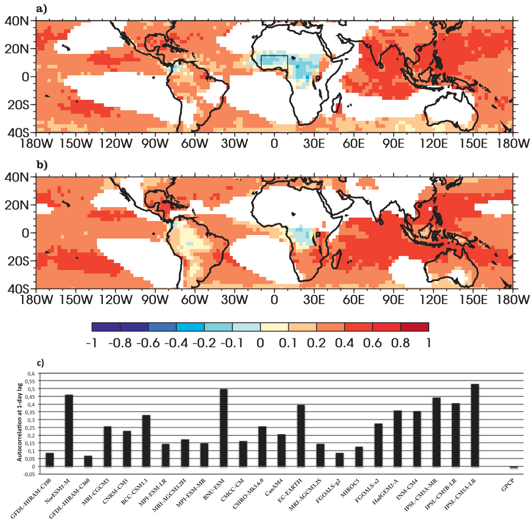
FIG. 16. Autocorrelation of (a) JAS and (b) December–February (DJF) 1–90-day filtered precipitation at a 1-day lag for the GPCP daily dataset. Only grid points where the mean precipitation was >1 \text{ mm day}^{-1} were considered. (c) Autocorrelation of 1–90-day filtered precipitation at a 1-day lag for GPCP and CMIP5 models averaged over the domain ( 5^{\circ}\text{--}15^{\circ}\text{N} , 10^{\circ}\text{W--}10^{\circ}\text{E} ). Autocorrelation was computed for each JAS season for 1997–2008 for GPCP and 1979–2008 for CMIP5 model, and then averaged over all years. CMIP5 models and the GPCP dataset were regridded on the NOAA OLR grid before any computations.
