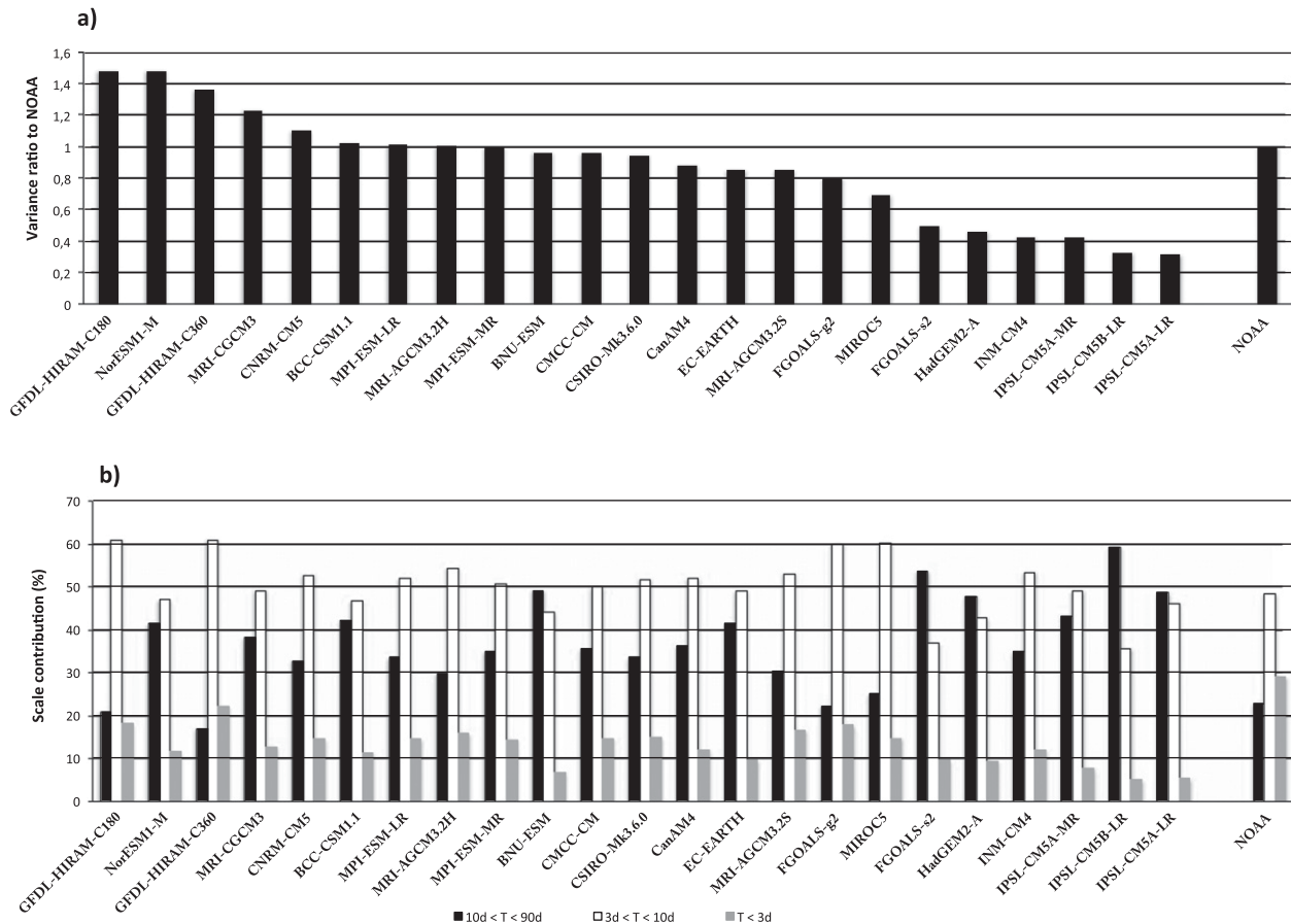
FIG. 15. (a) Variance of OLR in the 1–90-day band averaged over the domain ( 5^{\circ} – 20^{\circ} N, 10^{\circ} W– 10^{\circ} E) for the JAS season from 1979 to 2008. Values are normalized by the NOAA OLR variance. (b) Distribution of the OLR intraseasonal variance (%) across the 1–3-day (gray bars), 3–10-day (white bars), and 10–90-day (black bars) time scales.
