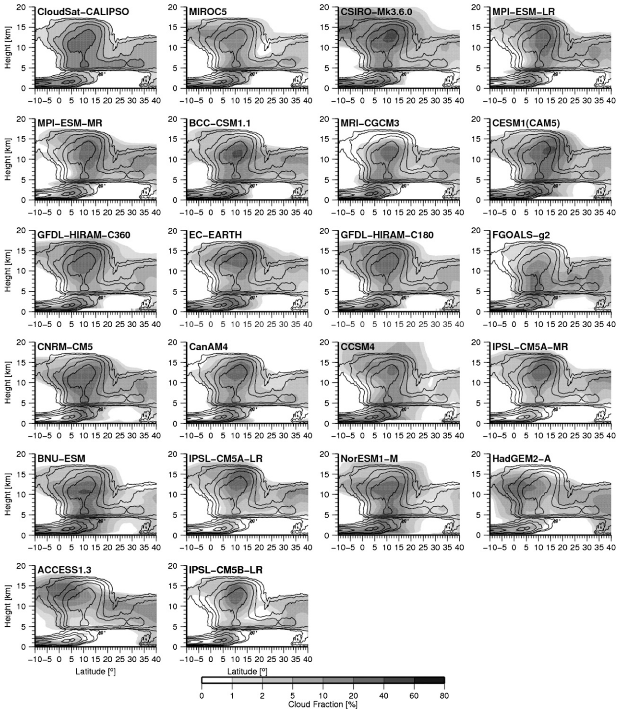
FIG. 8. Latitude–height plots of cloud fraction averaged between 10^{\circ}\text{W} and 10^{\circ}\text{E} for the JAS season for the years 2006–10 for the CloudSat–CALIPSO dataset and 1979–2008 for the models. Models are organized (top left)–(bottom right) from the warmest over the Sahara ( 20^{\circ} – 30^{\circ}\text{N} , 10^{\circ}\text{W} – 10^{\circ}\text{E} ) to the coldest.
