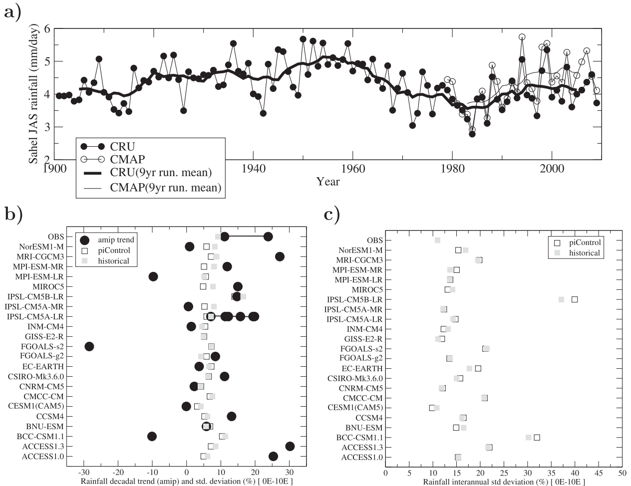
FIG. 3. (a) Time evolution of raw precipitation ( \text{mm day}^{-1} , lines with dots) averaged over ( 10^{\circ} – 18^{\circ}\text{N} , 0^{\circ} – 10^{\circ}\text{E} ) using CRU data (black dots) and CMAP (open dots), and its decadal component \bar{P}^9 (thick solid line), computed as the 9-yr running mean of the raw index. (b) Precipitation difference (%) between the 9-yr periods 2000–08 and 1979–87 for AMIP simulations (black dots) and standard deviation of \bar{P}^9 in historical (gray squares) and preindustrial control (open squares) experiments. The standard deviations (%) are computed on the full period (1850–2008) for historical simulations and on the available length for preindustrial simulations, which ranges from 250–1000 yr depending on the model. The standard deviation has been normalized by the mean \bar{P}^9 . For observations, the squares correspond to the normalized standard deviation of CRU \bar{P}^9 while the two black circles correspond to the precipitation difference (%) between the periods 2000–08 and 1979–87 in the CRU and CMAP observations. (c) Standard deviation of interannual fluctuation \delta P = P - \bar{P}^9 as a fraction of the mean precipitation (%), in preindustrial control (open squares) and historical (gray squares) experiments.
