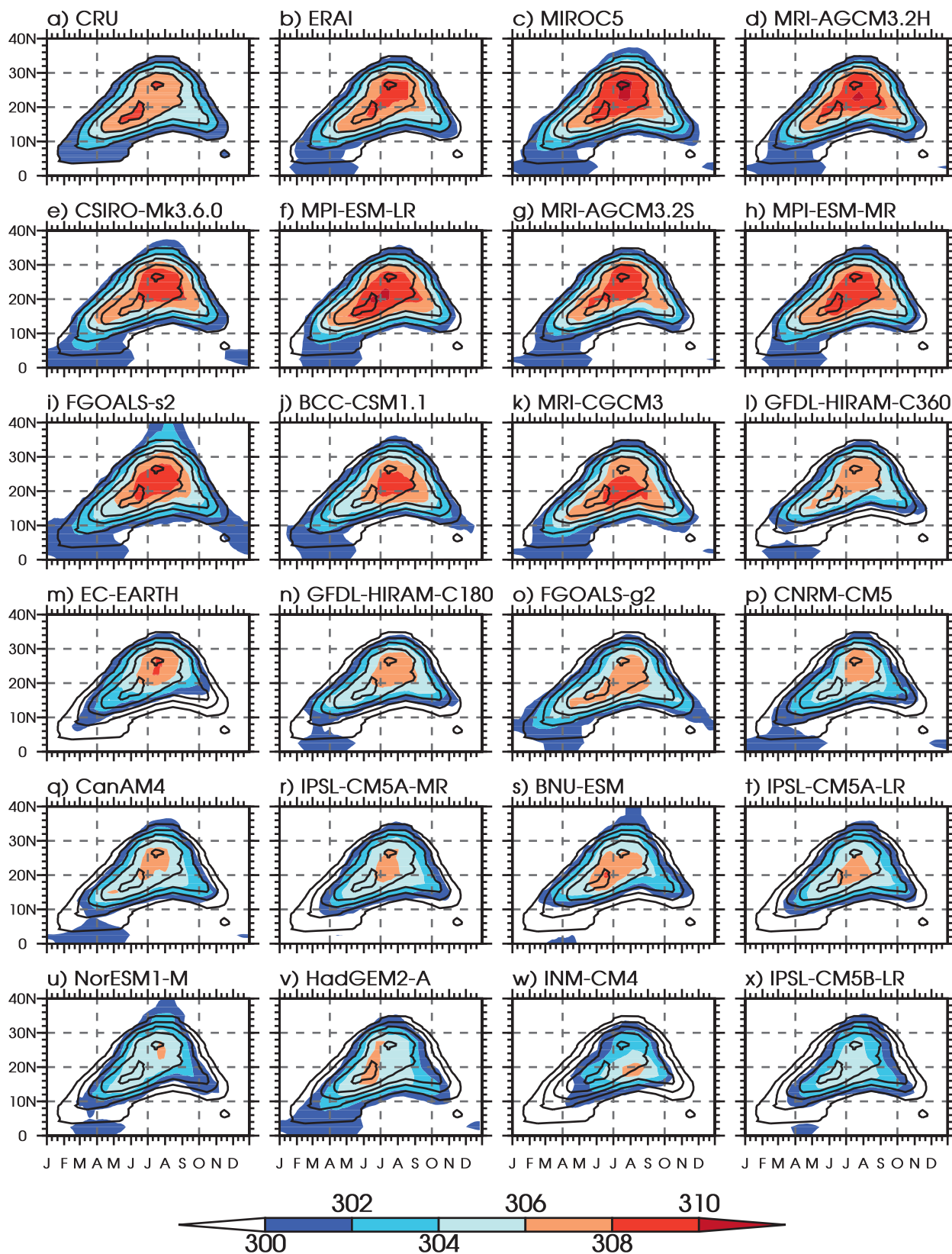
FIG. 13. As in Fig. 12, but for 2-m temperature (K).
