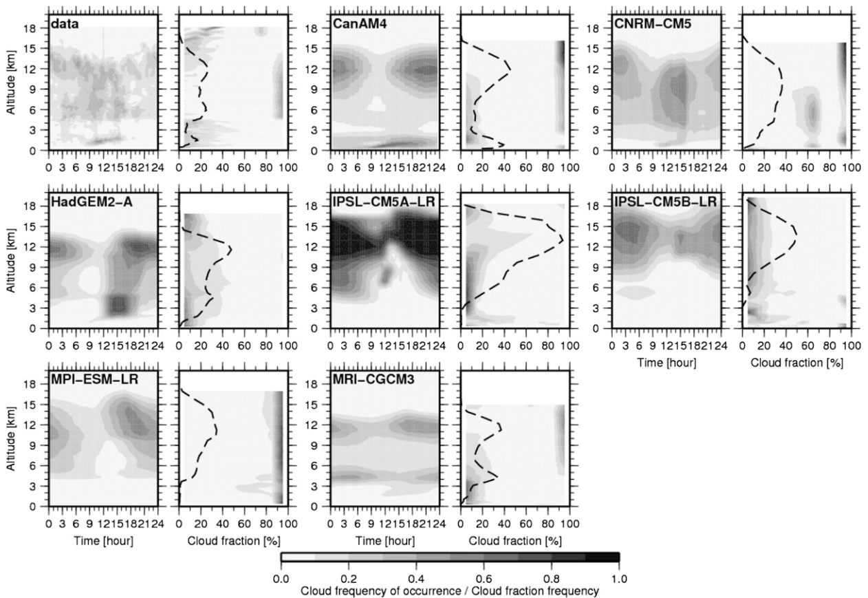
FIG. 18. As in Fig. 17, but for the August diurnal cycle of the cloud frequency of occurrence derived at the Niamey site (13.5°N, 2.2°E). Observations come from the AMF data acquired in 2006. The period 1979–2008 is used for the models. The vertical distribution of the cloud fraction is indicated in the right subpanels. It is normalized at each level by the total cloud frequency of occurrence (dashed line.)
