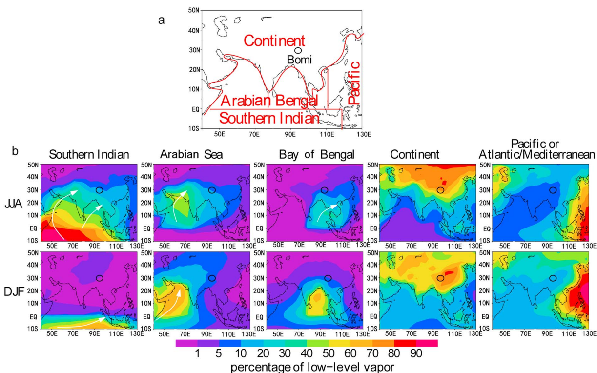
Figure 9. Water tagging experiment conducted using the zoomed LMDZiso model. (a) Definition of evaporative regions for water tagging. (b) Proportion of the JJA and DJF vapor originating from these different evaporative sources. The white arrows are an idealized representation of the dominant moisture flow. The open circle is a monitoring station in the TP (Bomi).
