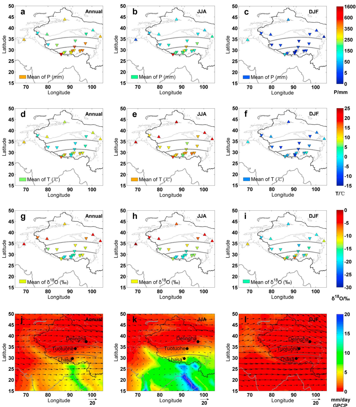
Figure 4. Spatial patterns of annual precipitation amount, temperature, and precipitation \delta^{18}\text{O} at precipitation stations, and the wind fields together with precipitation amount over the TP and surrounding regions. (a) Long-term averaged annual precipitation amount (mm) (triangles). (b and c) Same as Figure 4a but for JJA and DJF (triangles). (d) Long-term averaged annual temperature ( ^{\circ}\text{C} ). (e and f) Same as Figure 4d but for JJA and DJF. (g) Long-term averaged annual precipitation \delta^{18}\text{O} . (h and i) Same as Figure 4g but for JJA and DJF. (j) Composite of the annual mean wind fields (arrows) superimposed on the annual precipitation (mm/d, shading). (k and l) Same as Figure 4j but for JJA and DJF. Wind field data at 500 hPa are from the NCEP/NCAR reanalysis data (averaged from 1958 to 2007), and precipitation data are from the Global Precipitation Climatology Project (GPCP; http://www.esrl.noaa.gov/psd/data/gridded/data.gpcp.html ), averaged from 1979 to 2009. Up triangles stand for GNIP stations and down triangles for TNIP stations. The grey line shows the boundary where the elevation is above 3000 m. The dashed lines show the schematic boundaries separating the three domains (the westerlies domain, the transition domain, and the monsoon domain).
