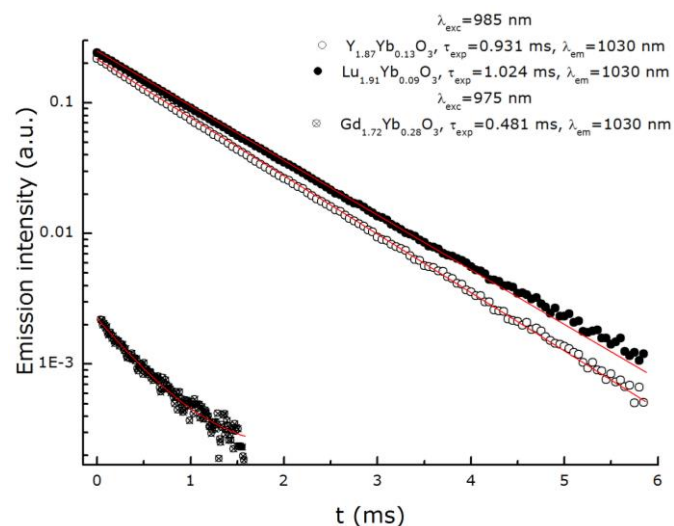
Fig. 4. Yb 3+ ions fluorescence decays in gadolinia, yttria and lutetia single crystals grown by the flux method, at λ em =1030 nm under λ exc =985 nm for the two latter and λ exc =975 nm for the former.
