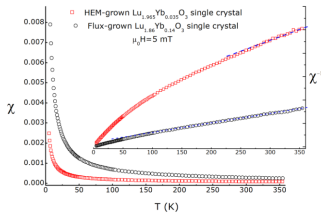
Fig. 3. MKSA magnetic susceptibility and inverse magnetic susceptibility of a Lu 1.86 Yb 0.14 O 3 flux-grown crystal and an HEM-grown Lu 1.965 Yb 0.035 O 3 crystal. The blue dashed line is a guide to visualize the Curie-Weiss behavior or what could potentially be interpreted in terms of such behavior.
