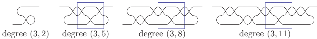
Figure 16: From D(1,0) to D(2,2,2,1,3)
