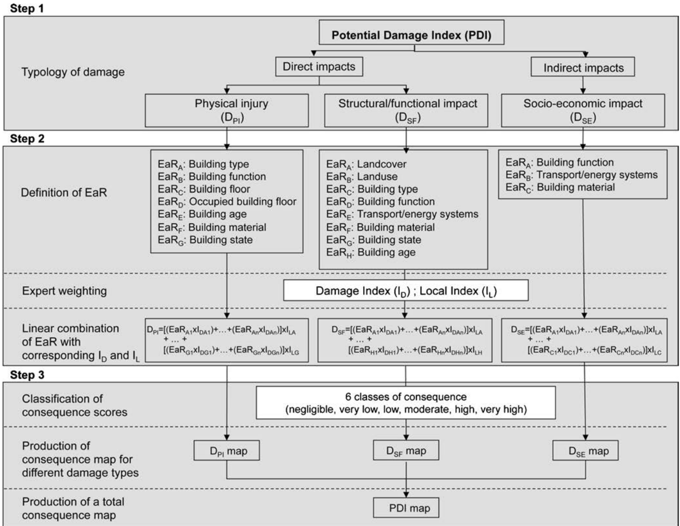
Fig. 5 Framework for the calculation of the Potential Damage Index (PDI) to estimate consequences at a regional scale
