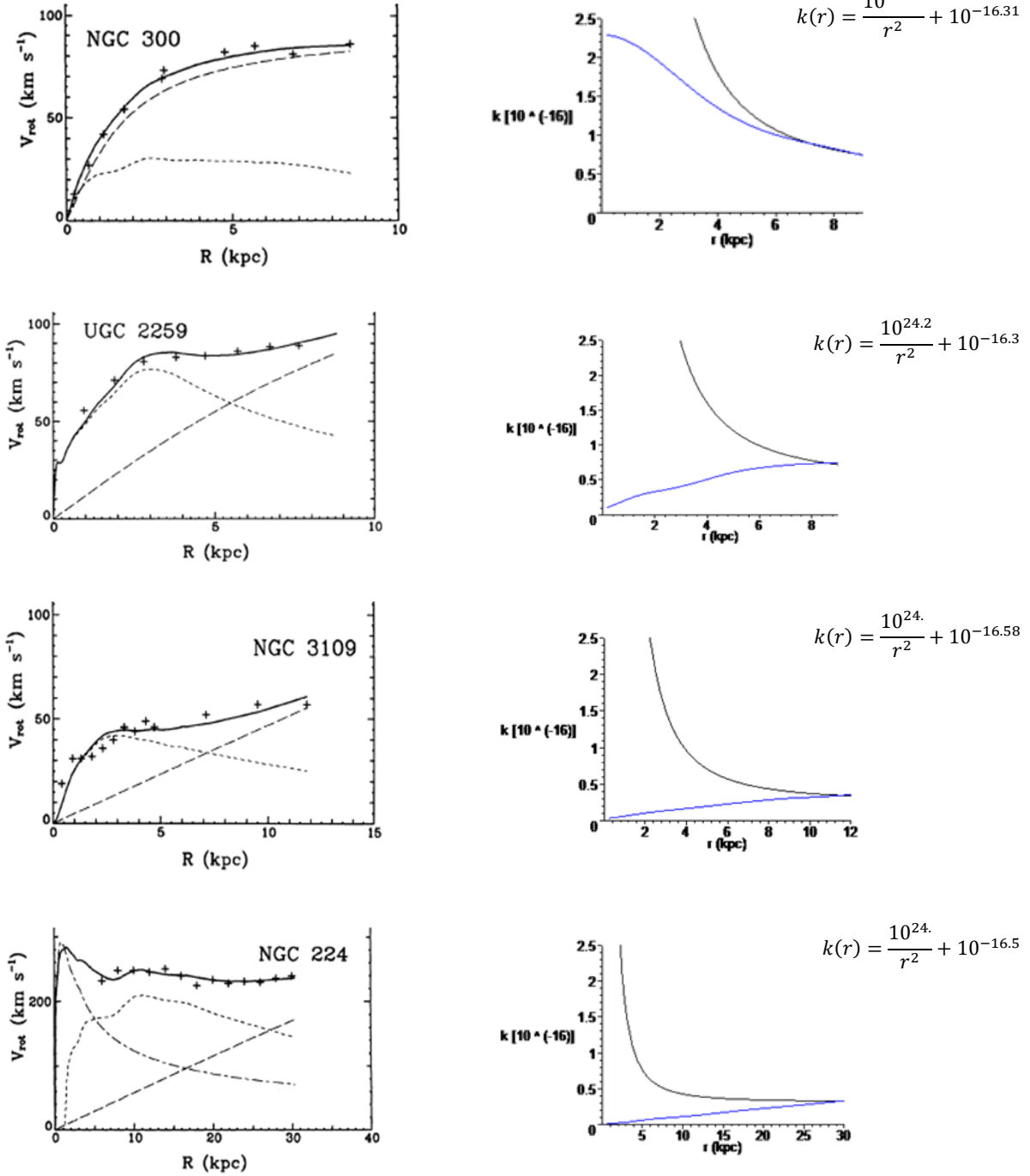
Fig. 8: Left graphs are the basis data from (KENT, 1987); right graphs represent k_{exp}(r) (in blue) and k(r) = \left(\frac{K_1}{r^2} + k_0\right) (in black) explaining ends of rotation speed curves (analytic expression of k(r) is given).
