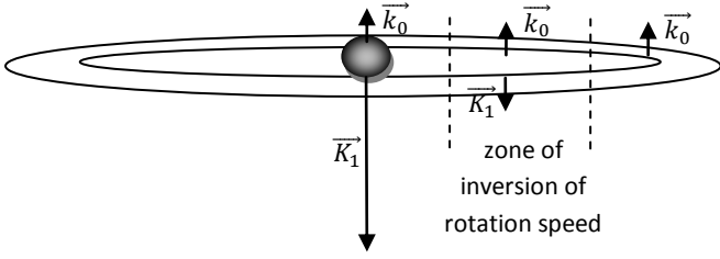
Fig. 11: Internal gravitic field \frac{K_1}{r^2} in opposite direction with external gravitic field k_0 implying two zones of opposite rotation speed.
