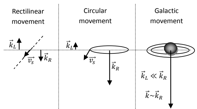
Fig. 3: Explanation of the orientation of \vec{k} in the cases of rectilinear, circular and galactic movement of matter galaxy
