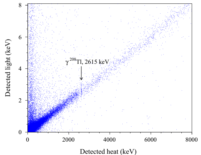
Fig. 5 The scatter plot of light versus detected heat based on the 13.7 mK data accumulated with the scintillating bolometer Zn^{100}MoO_4 , top , during 18.3 h of calibration measurements. The band populated by \gamma(\beta) events (below 2.6 MeV) and cosmic muons is clearly visible
