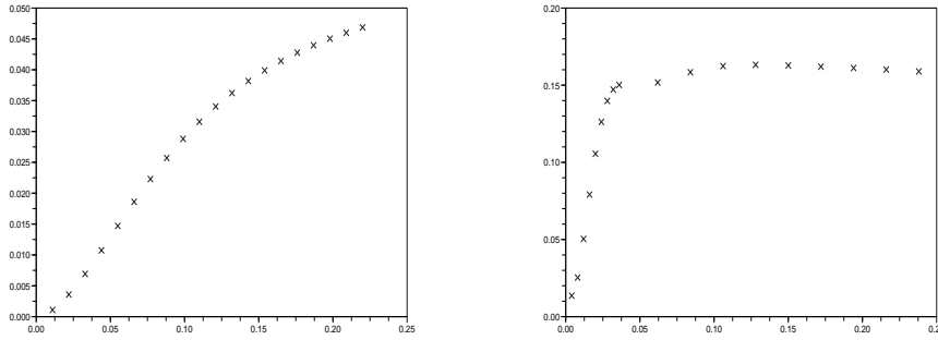
FIG. 5.2. l^2 error with respect to a between the limit functions associated to Kriging and corresponding asymptotical interpolatory subdivision schemes. Left, exponential case, right, Gaussian case. The crosses correspond to the different values of a for which the error has been evaluated.
