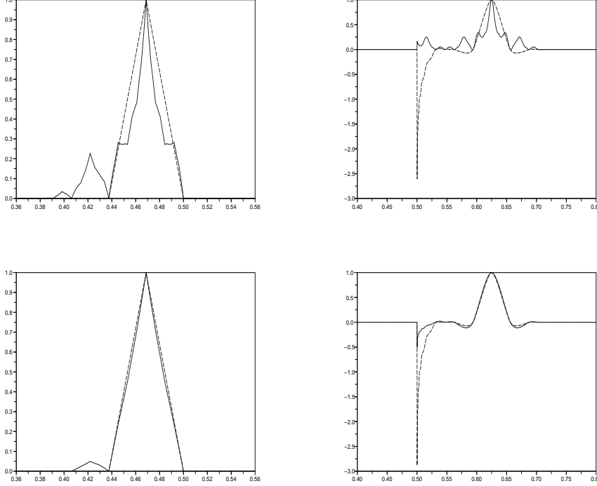
FIG. 5.1. Examples of limit functions associated to Kriging (solid line) and corresponding asymptotical interpolatory (dashed line) subdivision schemes. For sake of clarity, a zoom of these functions is performed by restriction to an interval containing their support. Left column, exponential case, m = 15 (Zone 1), from top to bottom, a = 0.2 , a = 0.04 . Right column, Gaussian case, m = 20 (Zone 2), from top to bottom, a = 0.2 , a = 0.02 .
