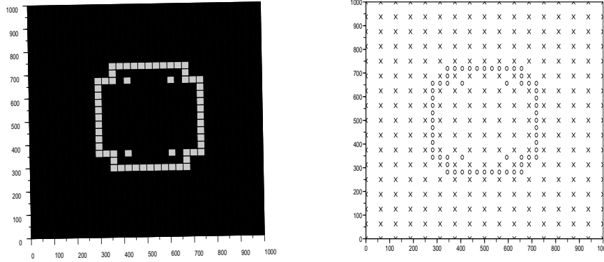
FIG. 5.6. Grid refinement. Left, estimation variance (\sigma^{J_0+1})^2 ( J_0 = 4 ) (the grey squares stand for the predicted points with an estimation variance larger than 0.014) , right, refined grid X^{J_0, J_0+1} (cross sign for the coarse grid and circle one for the 60 extra points corresponding to the grey squares of the left-hand plot).
