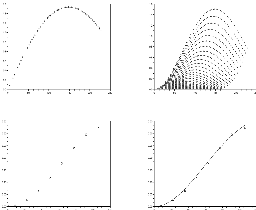
FIG. 3.2. The different steps of the semi-variogram identification. From top, left to bottom right, data (\{f_i\}_{i=0,\dots,N-1}) , variogram cloud (\{\frac{1}{2}(f_m - f_n)^2\}_{(m,n)\in(N-1)^2}) , experimental semi-variogram, identified semi-variogram model obtained by a least square fit.
