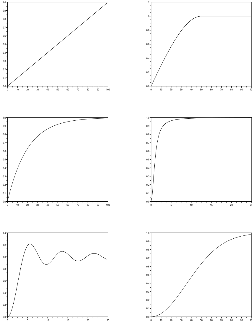
FIG. 3.1. Examples of valid models of semi-variograms. From top, left to bottom, right, linear ( \gamma(h) = \frac{h}{100} ), spherical ( \gamma(h) = \frac{3}{2} \frac{h}{50} - \frac{1}{2} \frac{h^3}{50^3} for h \leq 50 and 1, elsewhere), exponential ( \gamma(h) = 1 - e^{-\frac{1}{20}h} ), rational-quadratic ( \gamma(h) = \frac{h^2}{1+h^2} ), hole-effect ( \gamma(h) = 1 - 5 \frac{\sin(0.2h)}{h} ) and Gaussian ( \gamma(h) = 1 - e^{-\frac{1}{50^2}h^2} ) models.
