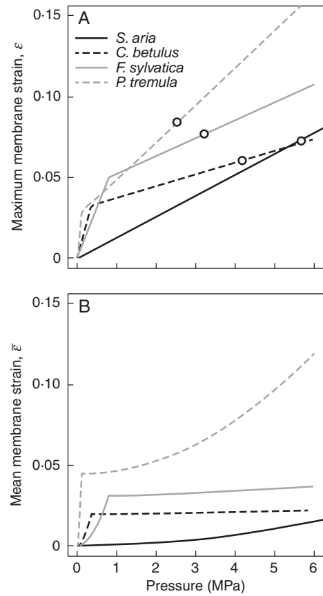
FIG. 6. Maximum pit membrane strain ( \epsilon_{\max} ) vs. pressure in four species with contrasting vulnerability to cavitation. Mean values of pit features were used to calculate pit membrane maximum ( \epsilon ) and mean ( \bar{\epsilon} ) strain in S. aria , C. betulus , F. sylvatica and P. tremula (as indicated in the key). The maximum strain occurs at the centre of the membrane, whereas the mean strain represents the relative increase in membrane length. Strains increase as the pit membrane is aspirated against the pit border. When the pit membrane reaches the pit border for a given pressure P_b , there is a breakpoint in the strain function. The P_b pressure differs between the species and can be deduced from the change in the slope of the strain function. Beyond this P_b value, only the pit membrane area that is unsupported by the aperture is deformed. The circles in (A) indicate the P_{50} values.
