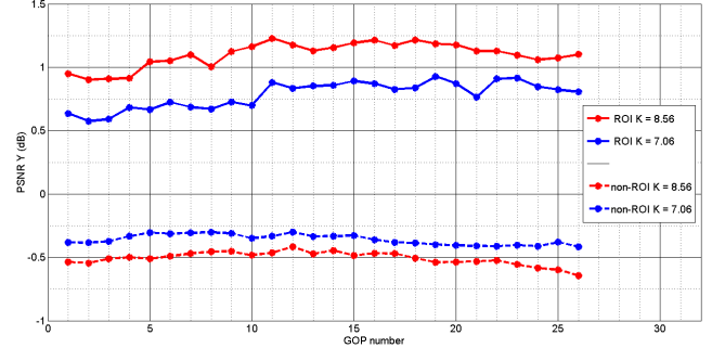
Fig. 6: \Delta\text{PSNR ROI} and non-ROI (dB) for the last 25 GOPs of FourPeople at 128kbps and using hierarchical bit allocation
