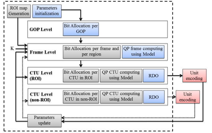
Fig. 4: ROI-based rate control scheme for HEVC
