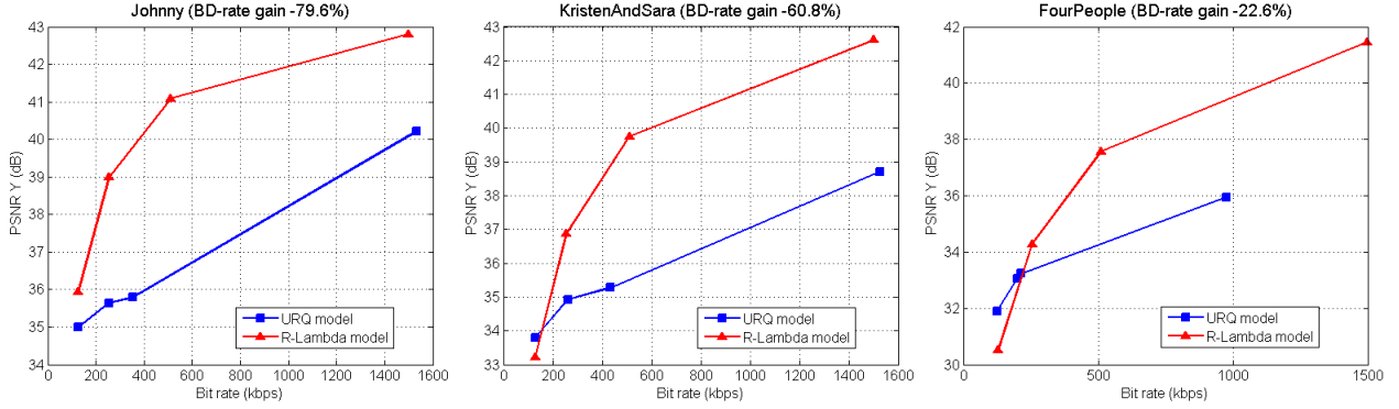
Fig. 2: R-D performances of R - \lambda algorithm, compared URQ model
