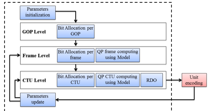
Fig. 1: Rate control scheme for HEVC
