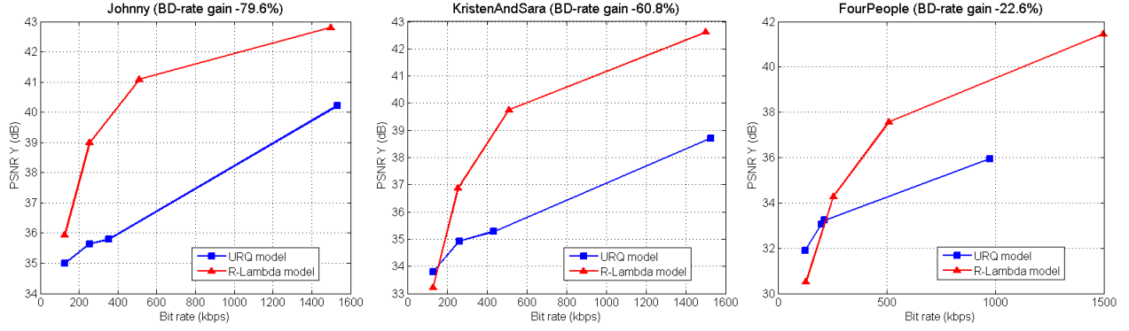
Fig. 2: R-D performances of R - \lambda algorithm, compared URQ model
