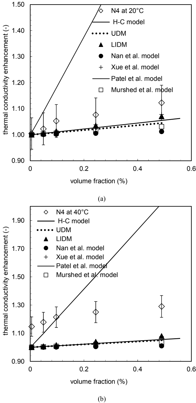
Figure 7. Relative TC enhancement of N4 in function of nanoparticle volume fraction at 20°C (a) and 40°C (b) – Comparison with theoretical correlations
