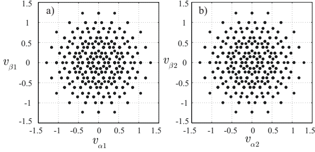
Fig. 2. Voltage vectors in the stator reference frame (normalized by V_{dc} = 2V_{dc1} = 2V_{dc2} ). Left: Subspace associated with the fundamental component (a). Right: Subspace associated with the third-harmonic component (b).
