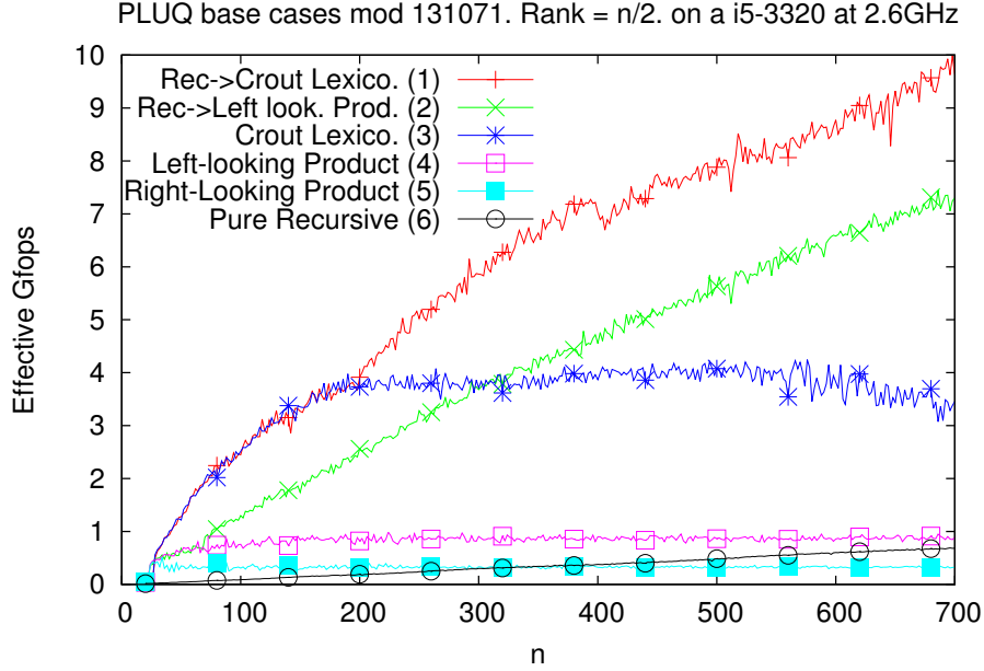
Figure 1: Computation speed of PLUQ decomposition base cases.
