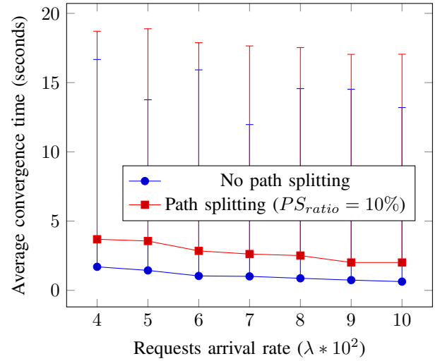
Fig. 7: Convergence time - Multicast requests
