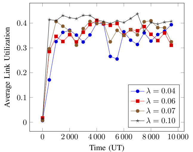
Fig. 4: Average link utilization - Multicast Requests
