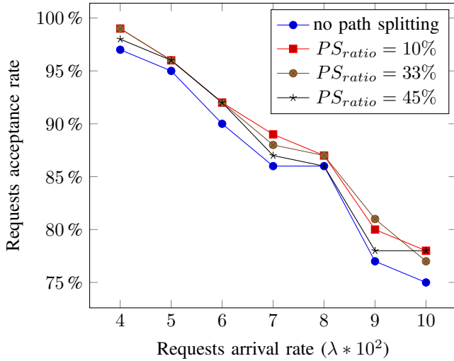
Fig. 8: Unicast requests acceptance rate for \beta = 1
