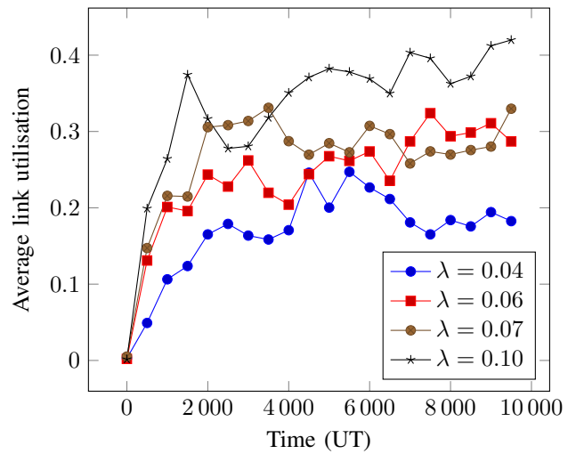
Fig. 3: Average link utilization - Unicast Requests
