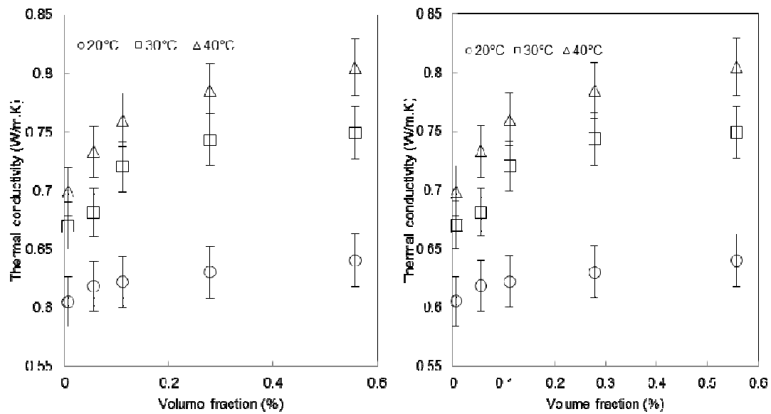
Figure 2. Thermal conductivity of N3 (left) and N4 (right) – Impact of CNT volume fraction and temperature
