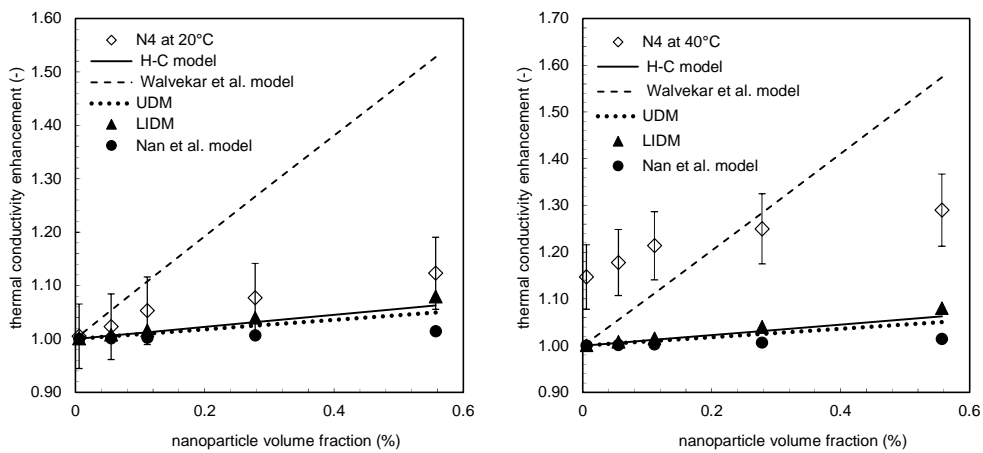
Figure 5. Relative TC enhancement of N 4 in function of nanoparticle volume fraction at 20°C (left) and 40°C (right) – Comparison with theoretical correlations
