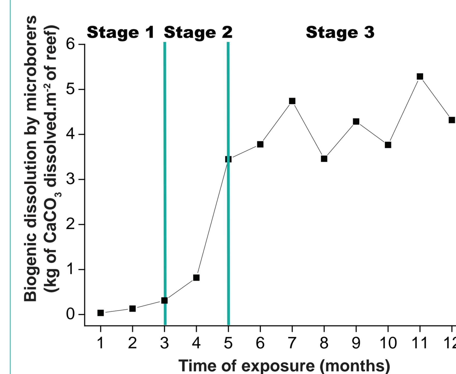
Figure 6: Biogenic dissolution by microborers expressed in kg of CaCO 3 dissolved per square meter of reef according to the time of exposure in months.
