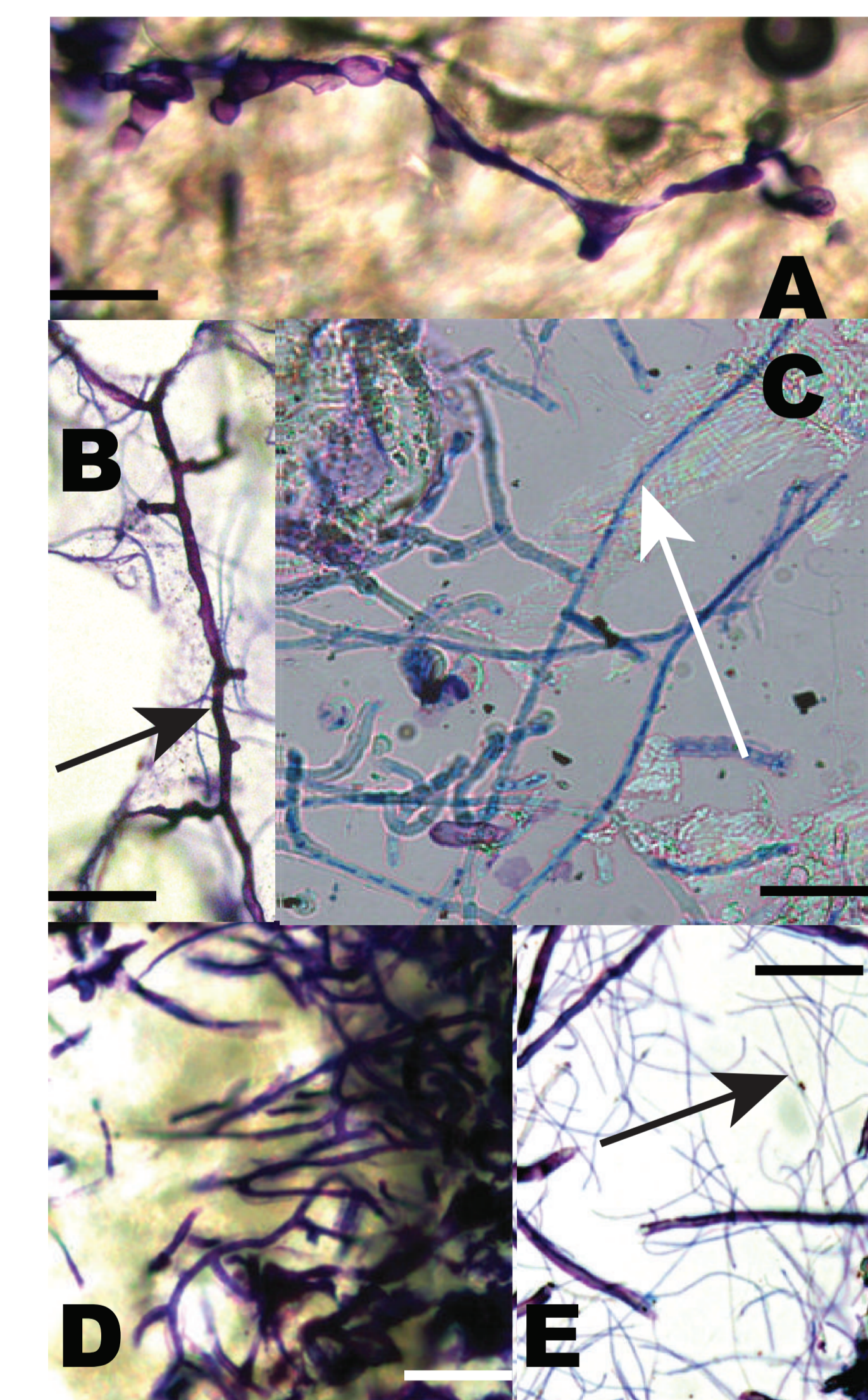
Figure 3: A- Phaeophila sp.; B- Ostreobium quekettii ; C- Hyella sp.; D- Mastigocoleus testarum ; E- Fungi or Plectonema terebrans . Scale bar = 40µm
