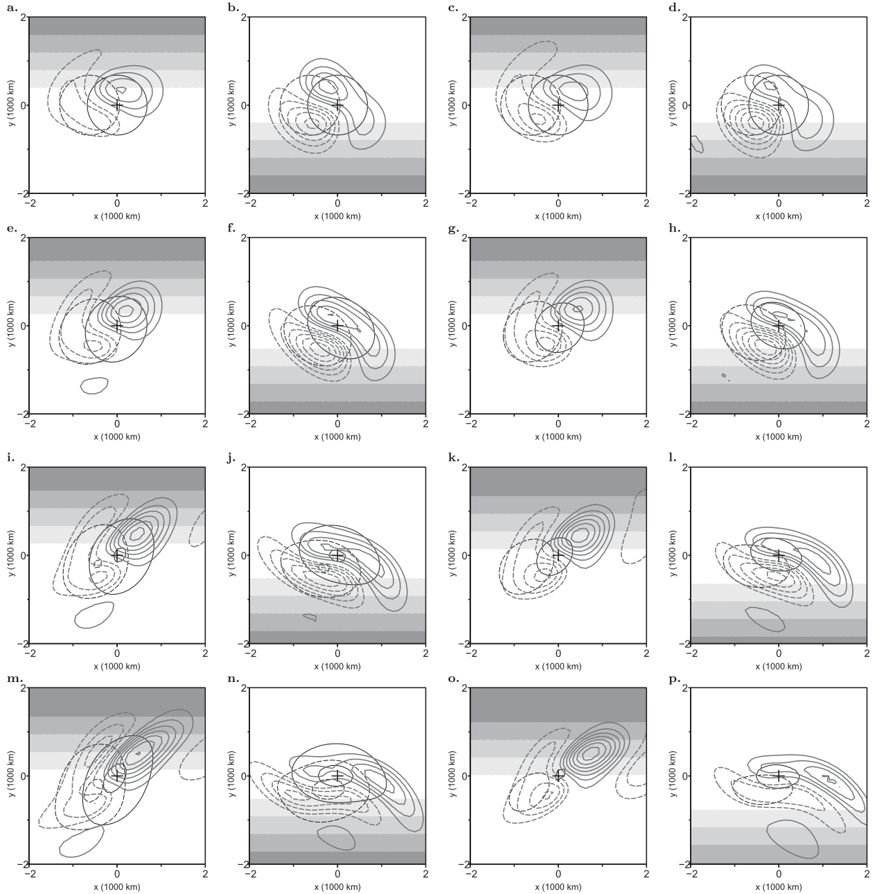
FIG. 4. Time evolution of the perturbation streamfunction at the lower (black solid contours) and upper (black dashed contours) layer and the stretching term -\lambda^{-1} s \omega'_{u-l} (gray contours) for (first column) an anticyclonic shear ( c^z = 1.0 , c_u^x = 1.0 , c_u^y = -0.5 ) without \beta , (second column) a cyclonic shear ( c^z = 1.0 , c_u^x = -1.0 , c_u^y = -0.5 ) without \beta , (third column) an anticyclonic shear ( c^z = 1.0 , c_u^x = 1.0 , c_u^y = 0.5 ) with \beta = 3\beta_0 , and (fourth column) a cyclonic shear ( c^z = 1.0 , c_u^x = 1.0 , c_u^y = 0.5 ) with \beta = 3\beta_0 . Shadings correspond to the basic-state zonal wind in the lower layer (positive values only). The different times (top to bottom) are t = 0.125 , t = 6 , t = 12 , and t = 18 h. Intervals as in Figs. 1 and 2.
