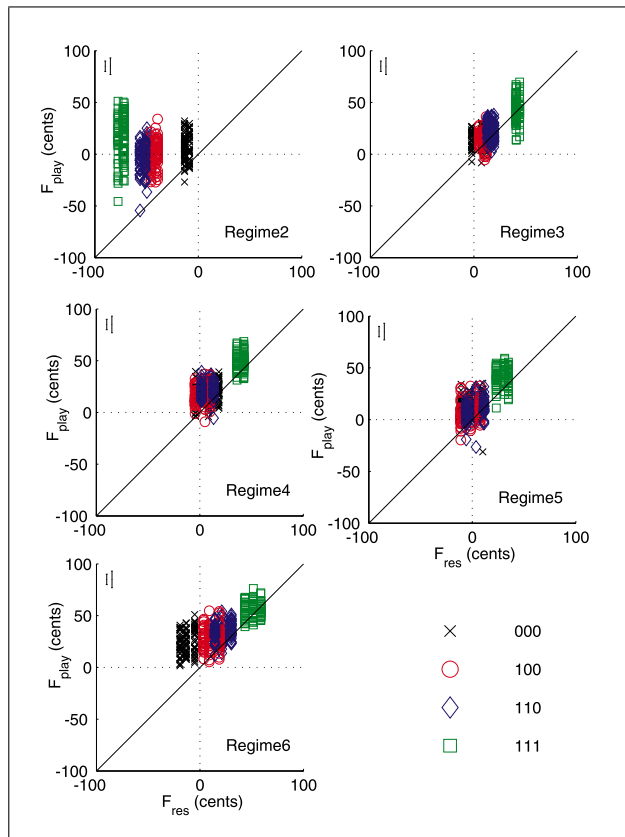
Figure 6. Playing frequencies ( F_{\text{play}} ) as functions of resonance frequencies ( F_{\text{res}} ), given in cents (taking the equally-tempered scale as a reference) for all the 2160 recorded notes. There is one figure for each regime, from regime 2 to regime 6, and a different marker for each fingering: 000 in crosses, 100 in circles, 110 in diamonds and 111 in squares. The error bar on the left represents twice the average standard deviation of a note. The error bar on the right represents twice the average reproducibility of the trumpet players.
