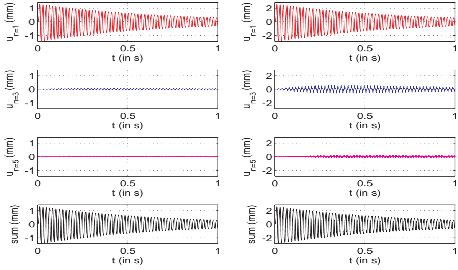
Figure 9: Simulation of Eq. (1) for f_{max}^1 = 5 N: linear approximation is correct since the amplitude of the transverse displacement is very small. For f_{max}^2 = 10 N, nonlinear effects begins to appear mainly for order 3.
