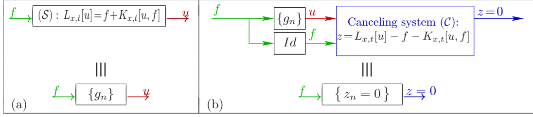
Figure 5: Canceling system and equivalence principle of Green-Volterra kernels.
