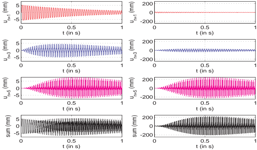
Figure 10: Simulation of Eq. (1) for f_{max}^3 = 20 N: the nonlinear responses have the same amplitude that the linear one, f_{max}^3 is roughly the convergence radius of the Volterra series. For f_{max}^4 = 40 N, the amplitude of the force is too high, the series does not converge anymore.
