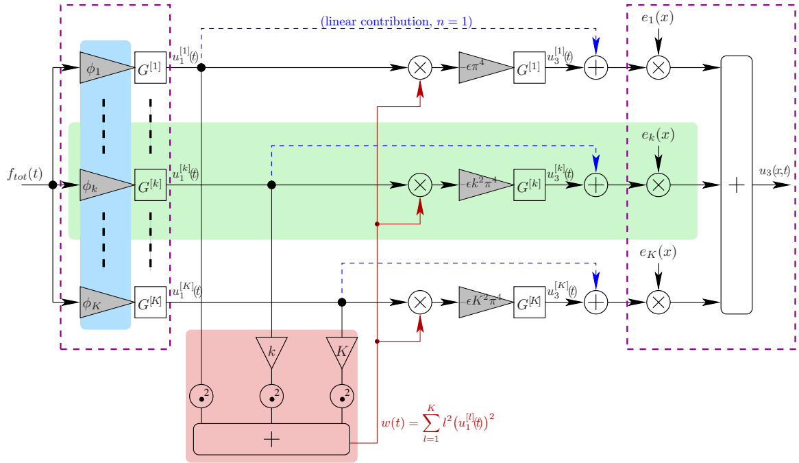
Figure 2: Block-diagram of an o(\epsilon) -simulation of Eq. (1) with K modes: the dashed arrows isolate the linear dynamics ( n=1 ) of each mode; the shaded central part isolates the o(\epsilon) -dynamics of a mode k ; the shaded bottom part isolates the dynamics of the integral term in Eq. (1); the shaded left part corresponds to simple gains, controlled by the spatial distribution of the excitation force. Note that the two dotted boxes correspond to those in Fig. 1 since \phi_k = \langle \phi, e_k \rangle_{L^2(\Omega)} .
