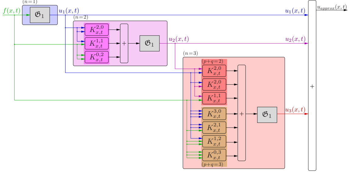
Figure 6: Realization of the three first orders of the general structure obtained from Eqs. (19-20), (29-30). In this structure, blocks K_{x,t}^{p,q} are the multilinear operators in Eq. (18), fed by the p+q signals, from top to bottom. Blocks (with no rounded corners) correspond to the linear operator \mathfrak{G}_1 associated with the Green's function g_1 , that is, \mathfrak{G}_1[w](x,t) = \int_{\Omega \times \mathbb{T}} g_1(x,t; \xi, \tau) w(\xi, \tau) d\xi d\tau .
