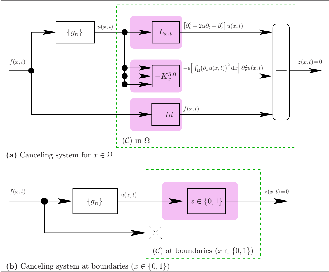
Figure 7: Block-diagram versions of Eq. (1) (sub-figure (a)) and of Eq. (2) (sub-figure (b)) for a general force f(x, t) . The associated canceling systems are delimited by dotted boxes.
