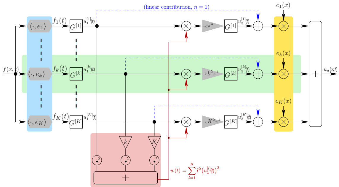
Figure 8: Block-diagram of an o(\epsilon) -simulation of Eq. (1) based on Green-Volterra kernels with K modes: the excitation force f(x, t) is completely unknown to the system and is decomposed on the modal basis using a scalar product.
