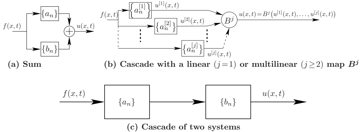
Figure 4: Interconnection laws of several Green-Volterra systems: (a) sum, (b) linear and multilinear maps, (c) cascade of two systems.
