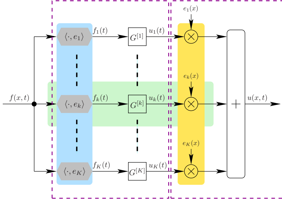
Figure 1: Block-diagram of the simulation of the linearized version of (1-3) with K modes. Symbol \otimes is a standard multiplication. More precisely, for functions with separated variables ( x \mapsto e_k(x) and t \mapsto u_k(t) ), it corresponds to the tensor product [e_k \otimes u_k](x, t) = e_k(x) u_k(t) as in Eq. (6).
