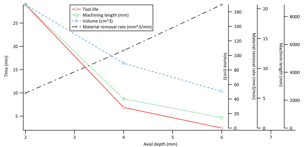
Fig. 21 Evolution of volume and material removal rate according to axial depth
