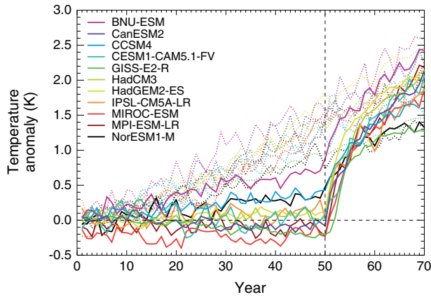
Figure 1. Evolution of annual mean anomaly of global mean near-surface air temperature (K) in the G2 simulations (solid lines) with respect to the long-term mean from each model’s CMIP5 piControl simulation. Time series from corresponding 1pctCO2 simulations are also shown (dotted lines). The termination of geoengineering in the G2 simulations is indicated by the dashed vertical line.
